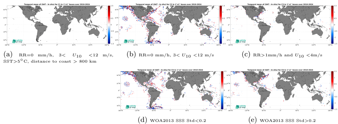
Figure 14: Temporal mean gridded over spatial boxes of size 1^\circ \times 1^\circ of \Delta\text{SSS} (SMOS SSS L2 v700 (ESA) - TSG (SAMOS)) for 5 different subdatasets corresponding to:RR=0 mm/h, 3 < U_{10} < 12 m/s, SST >5^\circ\text{C} , distance to coast > 800 km (a), RR=0 mm/h, 3 < U_{10} < 12 m/s (b), RR >1 mm/h and U_{10} < 4 m/s (c), WOA2013 SSS Std <0.2 (d), WOA2013 SSS Std >0.2 (e).
