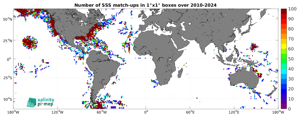
Figure 5: Number of SSS match-ups between TSG (SAMOS) SSS and the SMOS SSS L2 v700 (ESA) SSS product for the SMOS coastal zone (<800km) 60N-60S Pi-MEP region over 1^\circ \times 1^\circ boxes and for the full satellite product period.
