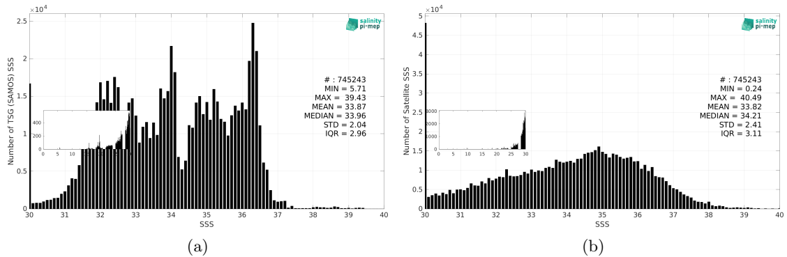
Figure 3: Histograms of SSS from TSG (SAMOS) (a) and SMOS SSS L2 v700 (ESA) (b) considering all match-up pairs per bins of 0.1 over the SMOS coastal zone (<800km) 60N-60S Pi-MEP region and for the full satellite product period.
