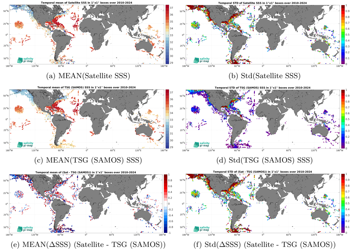
Figure 7: Temporal mean (left) and Std (right) of SSS from SMOS SSS L2 v700 (ESA) (top), TSG (SAMOS) (middle), and of \Delta SSS (Satellite - TSG (SAMOS)). Only match-up pairs are used to generate these maps.
