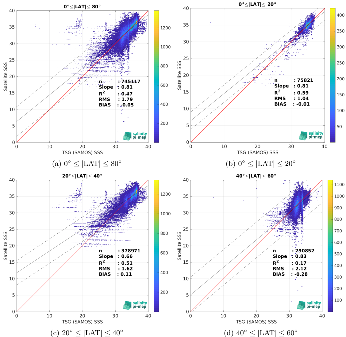
Figure 10: Contour maps of the concentration of SMOS SSS L2 v700 (ESA) SSS (y-axis) versus TSG (SAMOS) SSS (x-axis) at match-up pairs for different latitude bands. For each plot, the red line shows x=y . The black thin and dashed lines indicate a linear fit through the data cloud and the \pm 95\% confidence levels, respectively. The number match-up pairs n , the slope and R^2 coefficient of the linear fit, the root mean square (RMS) and the mean bias between satellite and in situ data are indicated for each latitude band in each plots.
