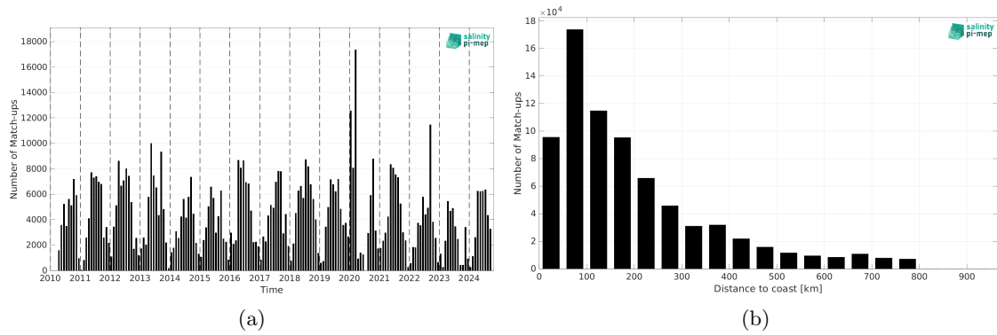
Figure 2: Number of match-ups between TSG (SAMOS) and SMOS SSS L2 v700 (ESA) SSS as a function of time (a) and as function of the distance to coast (b) over the SMOS coastal zone (<800km) 60N-60S Pi-MEP region and for the full satellite product period.
