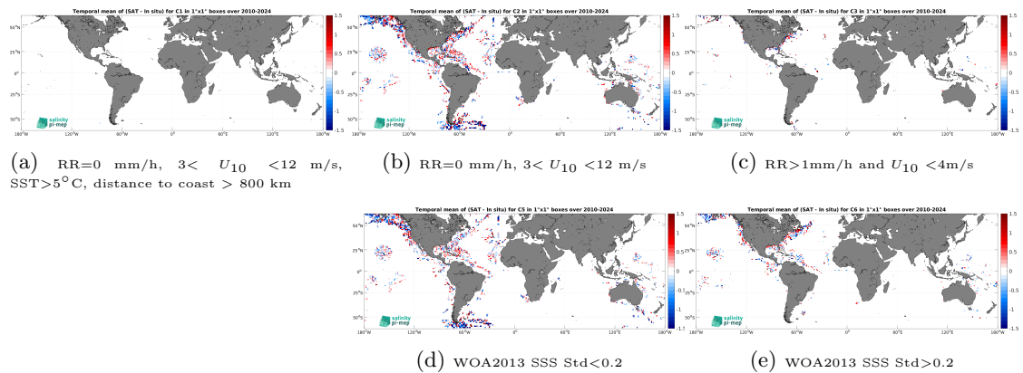
Figure 14: Temporal mean gridded over spatial boxes of size 1^\circ \times 1^\circ of \Delta SSS (SMOS SSS L2 v700 (ESA) - TSG (SAMOS)) for 5 different subdatasets corresponding to:RR=0 mm/h, 3 < U_{10} < 12 m/s, SST>5°C, distance to coast > 800 km (a), RR=0 mm/h, 3 < U_{10} < 12 m/s (b), RR>1mm/h and U_{10} < 4 m/s (c), WOA2013 SSS Std<0.2 (d), WOA2013 SSS Std>0.2 (e).
