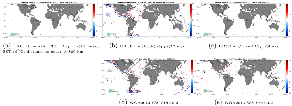
Figure 12: Temporal mean gridded over spatial boxes of size 1^\circ \times 1^\circ of \Delta SSS (SMOS SSS L2 v700 (ESA) - TSG (SAMOS)) for 5 different subdatasets corresponding to:RR=0 mm/h, 3 < U_{10} < 12 m/s, SST >5^\circ\text{C} , distance to coast > 800 km (a), RR=0 mm/h, 3 < U_{10} < 12 m/s (b), RR >1 mm/h and U_{10} < 4 m/s (c), WOA2013 SSS Std <0.2 (d), WOA2013 SSS Std >0.2 (e).
