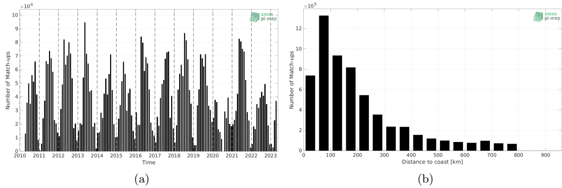
Figure 1: Number of match-ups between TSG (SAMOS) and SMOS SSS L2 v700 (ESA) SSS as a function of time (a) and as function of the distance to coast (b) over the SMOS coastal zone (<800km) 60N-60S Pi-MEP region and for the full satellite product period.
