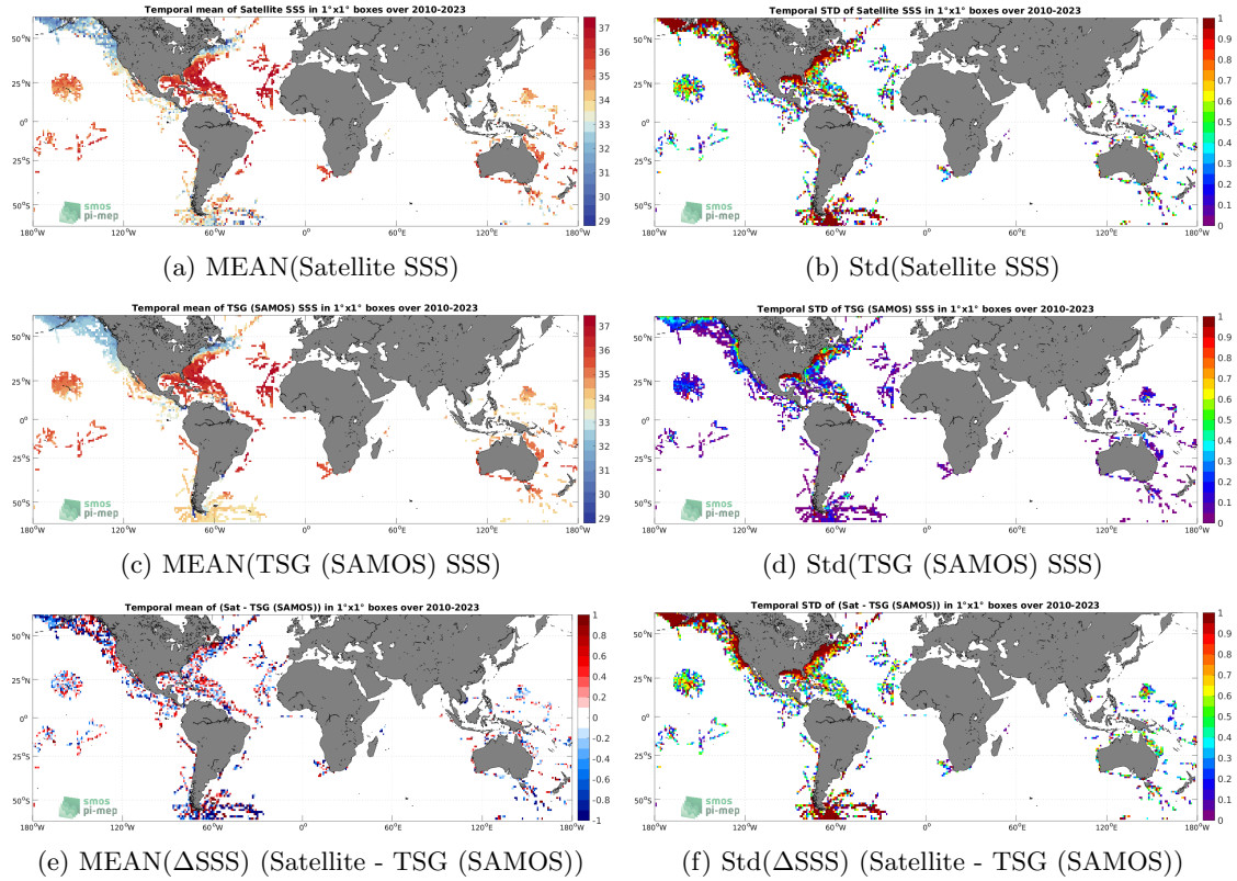
Figure 6: Temporal mean (left) and Std (right) of SSS from SMOS SSS L2 v700 (ESA) (top), TSG (SAMOS) (middle), and of \Delta SSS (Satellite - TSG (SAMOS)). Only match-up pairs are used to generate these maps.
