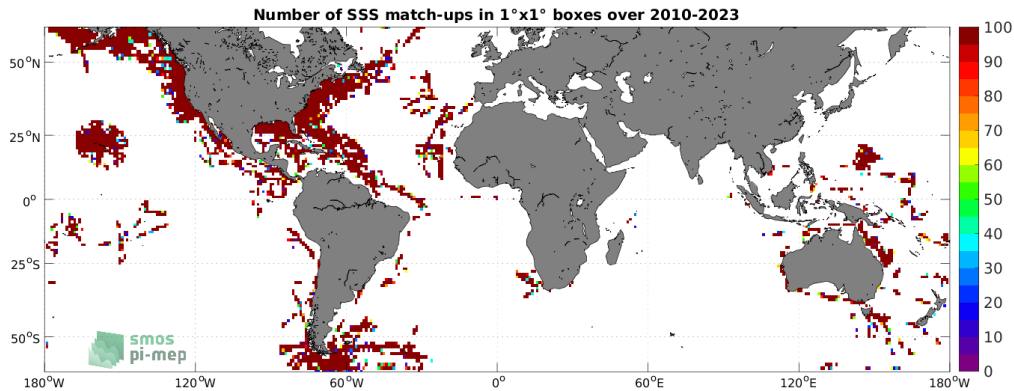
Figure 4: Number of SSS match-ups between TSG (SAMOS) SSS and the SMOS SSS L2 v700 (ESA) SSS product for the SMOS coastal zone (<800km) 60N-60S Pi-MEP region over 1^\circ \times 1^\circ boxes and for the full satellite product period.
