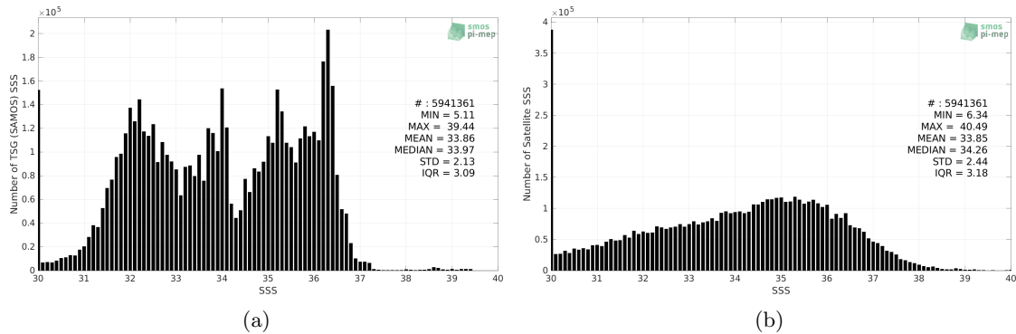
Figure 2: Histograms of SSS from TSG (SAMOS) (a) and SMOS SSS L2 v700 (ESA) (b) considering all match-up pairs per bins of 0.1 over the SMOS coastal zone (<800km) 60N-60S Pi-MEP region and for the full satellite product period.
