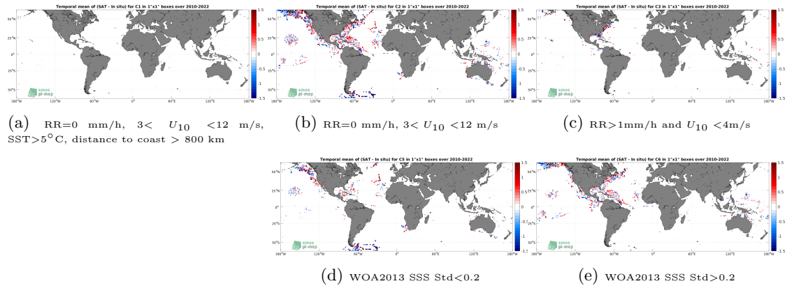
Figure 12: Temporal mean gridded over spatial boxes of size 1^\circ \times 1^\circ of \Delta\text{SSS} (SMOS SSS L2 v700 (ESA) - TSG (SAMOS)) for 5 different subdatasets corresponding to:RR=0 mm/h, 3 < U_{10} < 12 m/s, SST >5^\circ\text{C} , distance to coast > 800 km (a), RR=0 mm/h, 3 < U_{10} < 12 m/s (b), RR >1 mm/h and U_{10} < 4 m/s (c), WOA2013 SSS Std <0.2 (d), WOA2013 SSS Std >0.2 (e).
