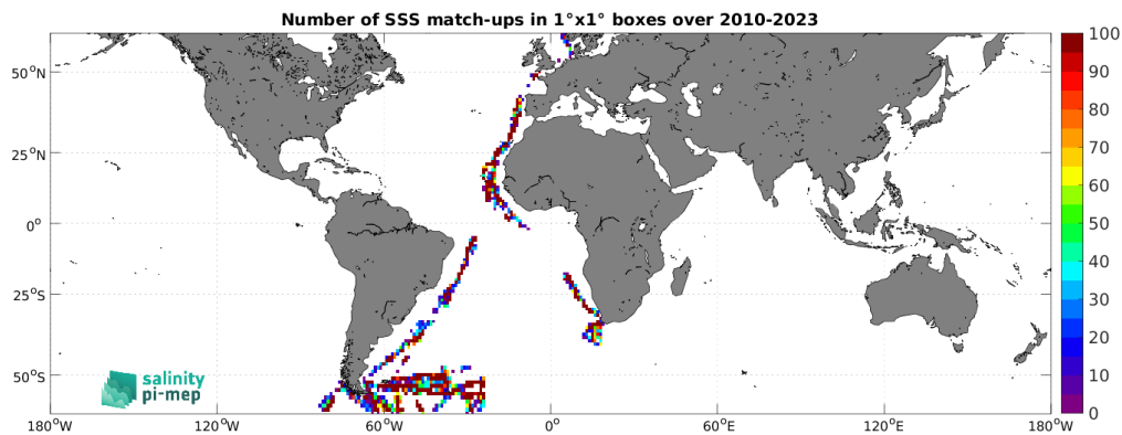
Figure 5: Number of SSS match-ups between TSG (Polarstern) SSS and the SMOS SSS L2 v700 (ESA) SSS product for the SMOS coastal zone (<800km) 60N-60S Pi-MEP region over 1^\circ \times 1^\circ boxes and for the full satellite product period.
