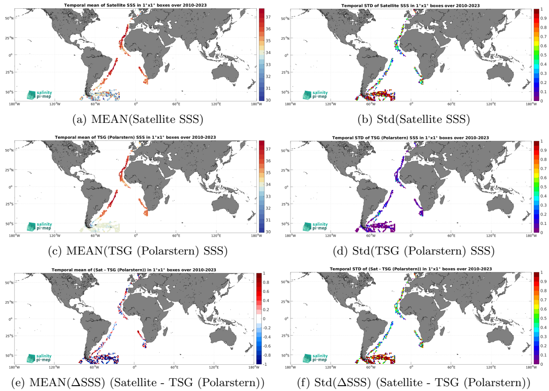
Figure 7: Temporal mean (left) and Std (right) of SSS from SMOS SSS L2 v700 (ESA) (top), TSG (Polarstern) (middle), and of \Delta SSS (Satellite - TSG (Polarstern)). Only match-up pairs are used to generate these maps.
