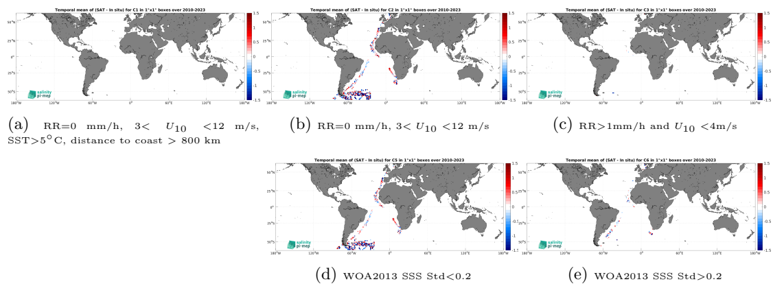
Figure 14: Temporal mean gridded over spatial boxes of size 1^\circ \times 1^\circ of \Delta\text{SSS} (SMOS SSS L2 v700 (ESA) - TSG (Polarstern)) for 5 different subdatasets corresponding to:RR=0 mm/h, 3 < U_{10} < 12 m/s, SST>5°C, distance to coast > 800 km (a), RR=0 mm/h, 3 < U_{10} < 12 m/s (b), RR>1mm/h and U_{10} < 4 m/s (c), WOA2013 SSS Std<0.2 (d), WOA2013 SSS Std>0.2 (e).
