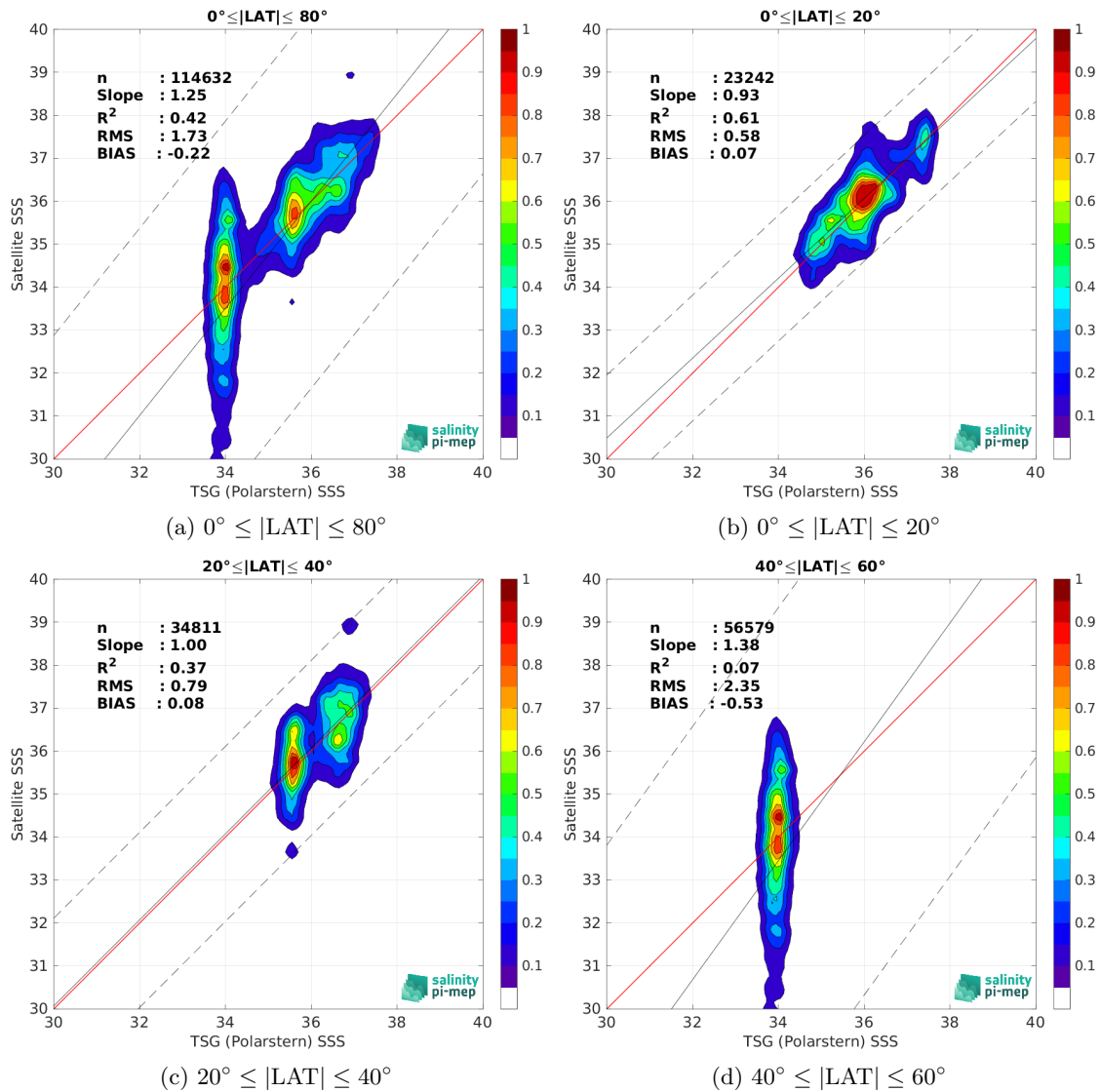
Figure 10: Contour maps of the concentration of SMOS SSS L2 v700 (ESA) SSS (y-axis) versus TSG (Polarstern) SSS (x-axis) at match-up pairs for different latitude bands. For each plot, the red line shows x=y . The black thin and dashed lines indicate a linear fit through the data cloud and the \pm 95\% confidence levels, respectively. The number match-up pairs n , the slope and R^2 coefficient of the linear fit, the root mean square (RMS) and the mean bias between satellite and in situ data are indicated for each latitude band in each plots.
