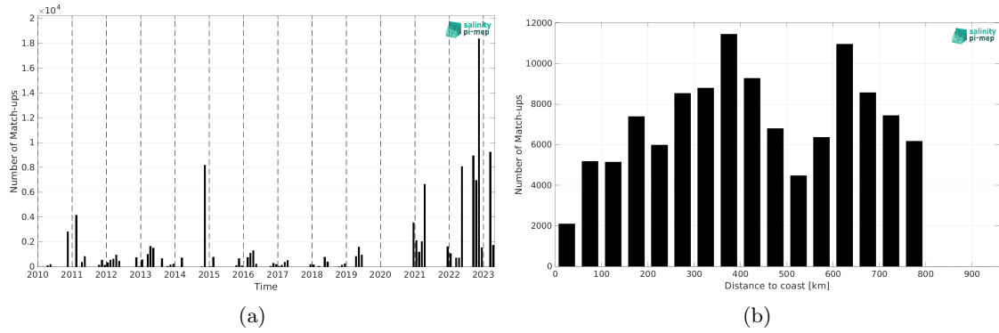
Figure 2: Number of match-ups between TSG (Polarstern) and SMOS SSS L2 v700 (ESA) SSS as a function of time (a) and as function of the distance to coast (b) over the SMOS coastal zone (<800km) 60N-60S Pi-MEP region and for the full satellite product period.
