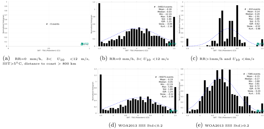
Figure 15: Normalized histogram of \Delta SSS (SMOS SSS L2 v700 (ESA) - TSG (Polarstern)) for 5 different subdatasets corresponding to: RR=0 mm/h, 3 < U_{10} < 12 m/s, SST > 5°C, distance to coast > 800 km (a), RR=0 mm/h, 3 < U_{10} < 12 m/s (b), RR > 1mm/h and U_{10} < 4 m/s (c), WOA2013 SSS Std < 0.2 (d), WOA2013 SSS Std > 0.2 (e).
