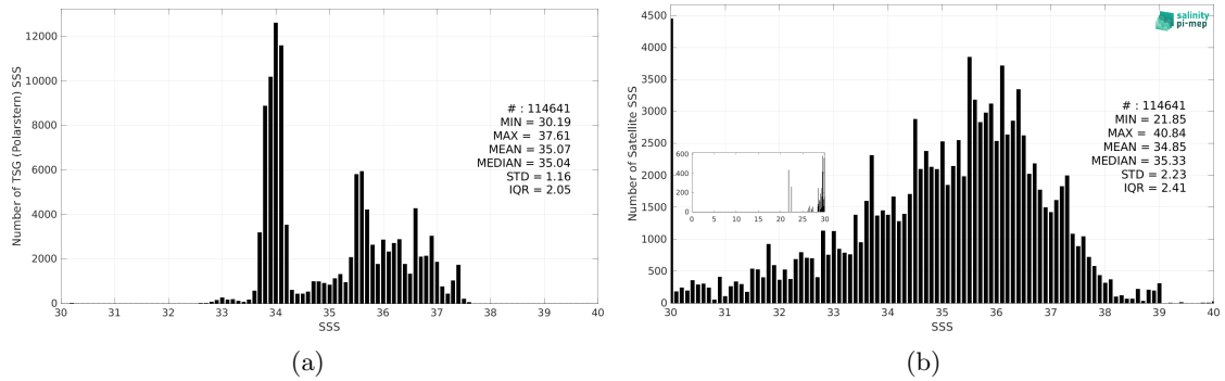
Figure 3: Histograms of SSS from TSG (Polarstern) (a) and SMOS SSS L2 v700 (ESA) (b) considering all match-up pairs per bins of 0.1 over the SMOS coastal zone (<800km) 60N-60S Pi-MEP region and for the full satellite product period.
