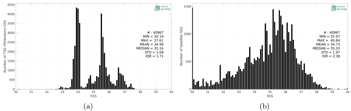
Figure 2: Histograms of SSS from TSG (Polarstern) (a) and SMOS SSS L2 v700 (ESA) (b) considering all match-up pairs per bins of 0.1 over the SMOS coastal zone (<800km) 60N-60S Pi-MEP region and for the full satellite product period.
