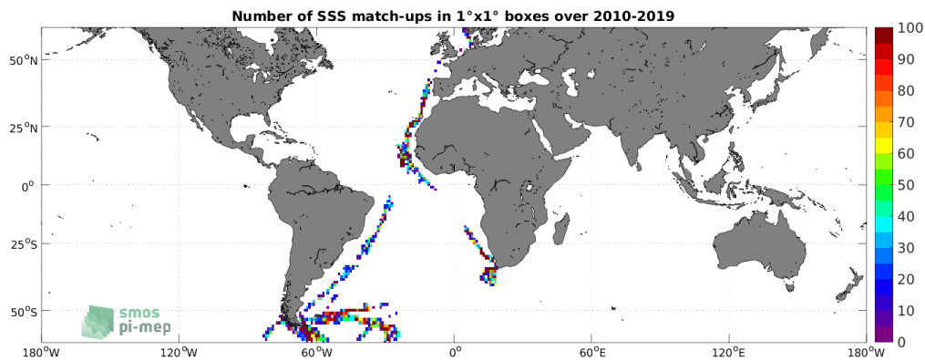
Figure 4: Number of SSS match-ups between TSG (Polarstern) SSS and the SMOS SSS L2 v700 (ESA) SSS product for the SMOS coastal zone (<800km) 60N-60S Pi-MEP region over 1^\circ \times 1^\circ boxes and for the full satellite product period.
