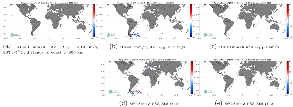
Figure 12: Temporal mean gridded over spatial boxes of size 1^\circ \times 1^\circ of \Delta\text{SSS} (SMOS SSS L2 v700 (ESA) - TSG (Polarstern)) for 5 different subdatasets corresponding to:RR=0 mm/h, 3 < U_{10} < 12 m/s, SST >5^\circ\text{C} , distance to coast > 800 km (a), RR=0 mm/h, 3 < U_{10} < 12 m/s (b), RR >1 mm/h and U_{10} < 4 m/s (c), WOA2013 SSS Std <0.2 (d), WOA2013 SSS Std >0.2 (e).
