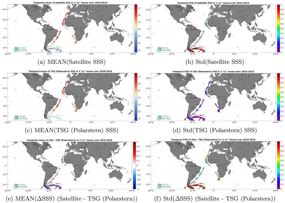
Figure 6: Temporal mean (left) and Std (right) of SSS from SMOS SSS L2 v700 (ESA) (top), TSG (Polarstern) (middle), and of \Delta SSS (Satellite - TSG (Polarstern)). Only match-up pairs are used to generate these maps.
