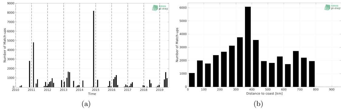
Figure 1: Number of match-ups between TSG (Polarstern) and SMOS SSS L2 v700 (ESA) SSS as a function of time (a) and as function of the distance to coast (b) over the SMOS coastal zone (<800km) 60N-60S Pi-MEP region and for the full satellite product period.
