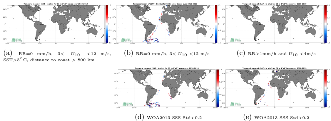
Figure 12: Temporal mean gridded over spatial boxes of size 1^\circ \times 1^\circ of \Delta SSS (SMOS SSS L2 v700 (ESA) - TSG (Polarstern)) for 5 different subdatasets corresponding to: RR=0 mm/h, 3 < U_{10} < 12 m/s, SST > 5°C, distance to coast > 800 km (a), RR=0 mm/h, 3 < U_{10} < 12 m/s (b), RR > 1mm/h and U_{10} < 4 m/s (c), WOA2013 SSS Std < 0.2 (d), WOA2013 SSS Std > 0.2 (e).
