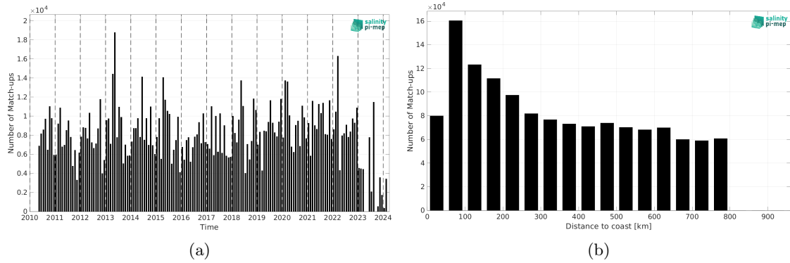
Figure 2: Number of match-ups between TSG (LEGOS-DM) and SMOS SSS L2 v700 (ESA) SSS as a function of time (a) and as function of the distance to coast (b) over the SMOS coastal zone (<800km) 60N-60S Pi-MEP region and for the full satellite product period.
