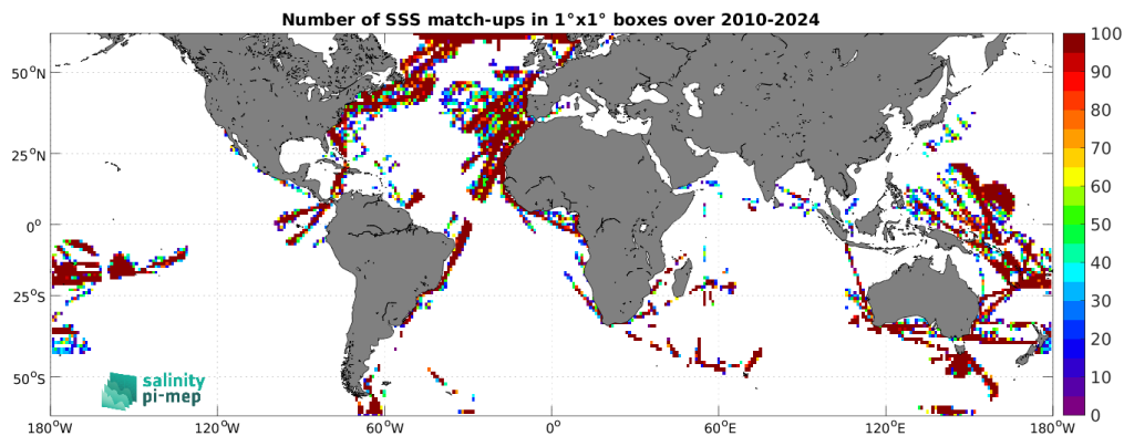
Figure 5: Number of SSS match-ups between TSG (LEGOS-DM) SSS and the SMOS SSS L2 v700 (ESA) SSS product for the SMOS coastal zone (<800km) 60N-60S Pi-MEP region over 1^\circ \times 1^\circ boxes and for the full satellite product period.
