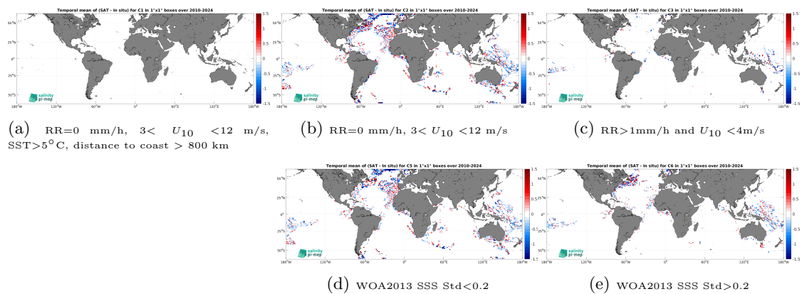
Figure 14: Temporal mean gridded over spatial boxes of size 1^\circ \times 1^\circ of \Delta\text{SSS} (SMOS SSS L2 v700 (ESA) - TSG (LEGOS-DM)) for 5 different subdatasets corresponding to:RR=0 mm/h, 3 < U_{10} < 12 m/s, SST>5°C, distance to coast > 800 km (a), RR=0 mm/h, 3 < U_{10} < 12 m/s (b), RR>1mm/h and U_{10} < 4 m/s (c), WOA2013 SSS Std<0.2 (d), WOA2013 SSS Std>0.2 (e).
