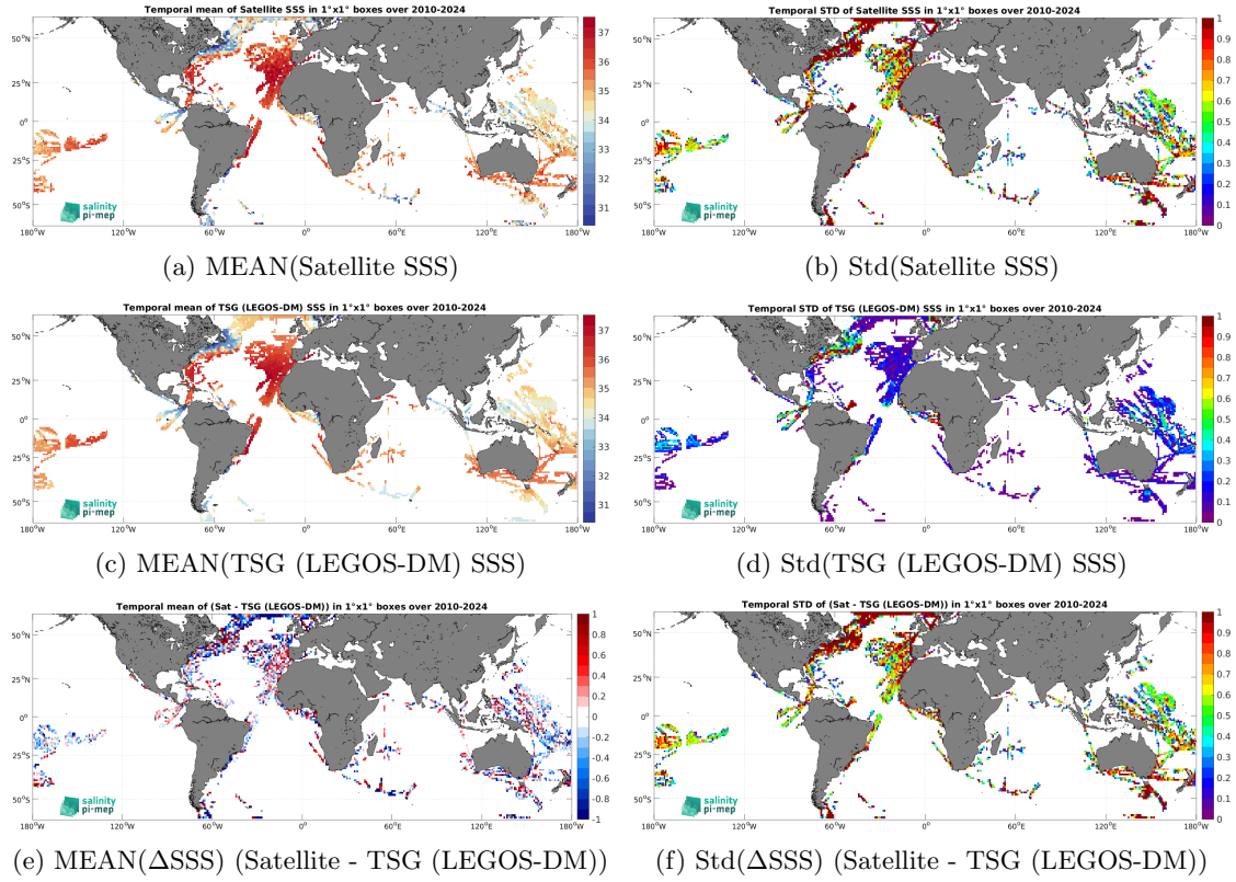
Figure 7: Temporal mean (left) and Std (right) of SSS from SMOS SSS L2 v700 (ESA) (top), TSG (LEGOS-DM) (middle), and of \Delta SSS (Satellite - TSG (LEGOS-DM)). Only match-up pairs are used to generate these maps.
