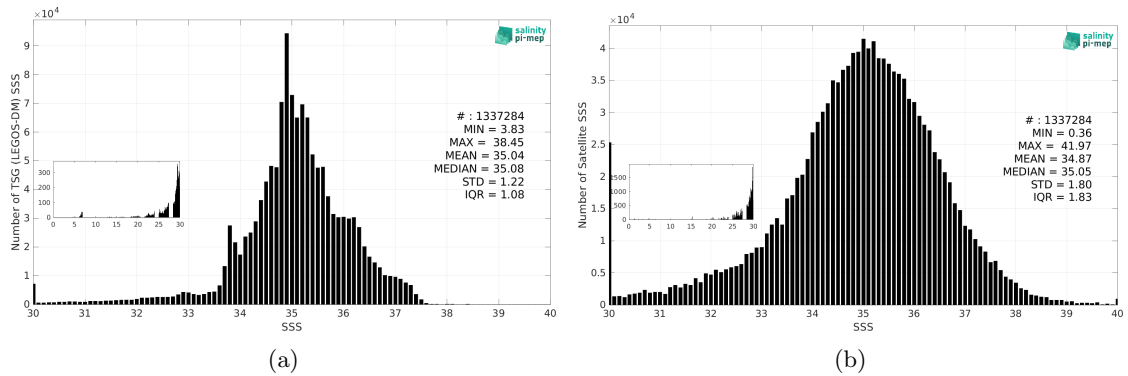
Figure 3: Histograms of SSS from TSG (LEGOS-DM) (a) and SMOS SSS L2 v700 (ESA) (b) considering all match-up pairs per bins of 0.1 over the SMOS coastal zone (<800km) 60N-60S Pi-MEP region and for the full satellite product period.
