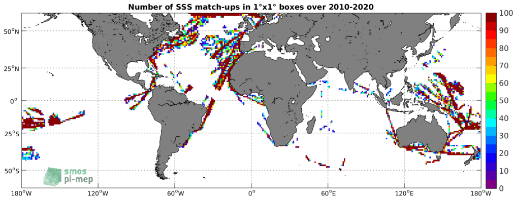
Figure 4: Number of SSS match-ups between TSG (LEGOS-DM) SSS and the SMOS SSS L2 v700 (ESA) SSS product for the SMOS coastal zone (<800km) 60N-60S Pi-MEP region over 1°x1° boxes and for the full satellite product period.
