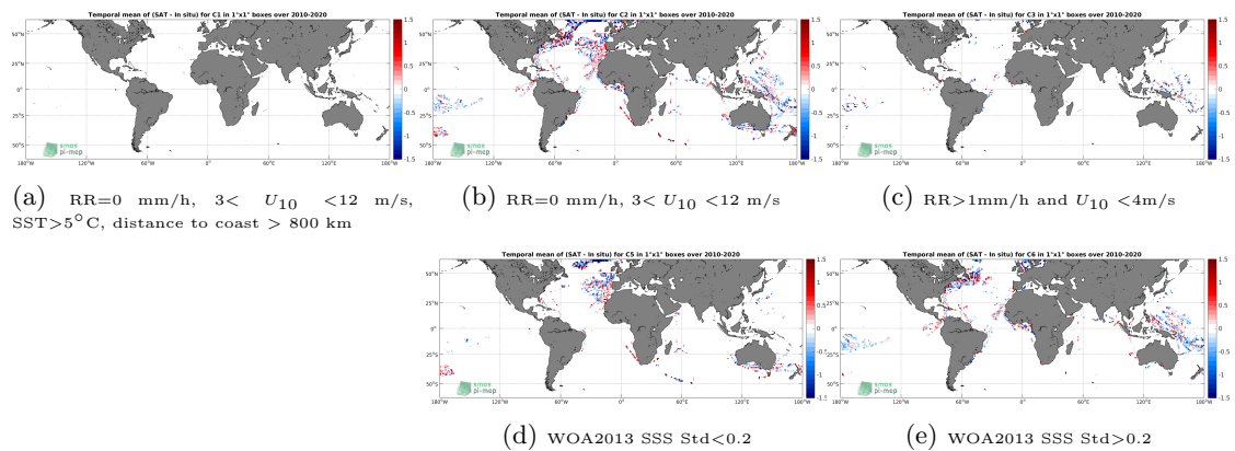
Figure 12: Temporal mean gridded over spatial boxes of size 1^\circ \times 1^\circ of \Delta SSS (SMOS SSS L2 v700 (ESA) - TSG (LEGOS-DM)) for 5 different subdatasets corresponding to: RR=0 mm/h, 3 < U_{10} < 12 m/s, SST > 5^\circ\text{C} , distance to coast > 800 km (a), RR=0 mm/h, 3 < U_{10} < 12 m/s (b), RR > 1 mm/h and U_{10} < 4 m/s (c), WOA2013 SSS Std < 0.2 (d), WOA2013 SSS Std > 0.2 (e).
