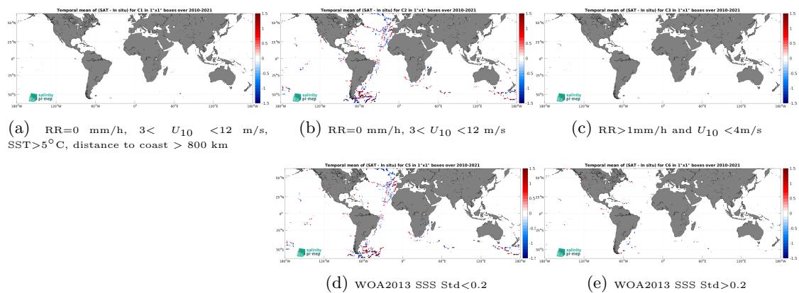
Figure 14: Temporal mean gridded over spatial boxes of size 1^\circ \times 1^\circ of \Delta SSS (SMOS SSS L2 v700 (ESA) - TSG (GOSUD-Sailing-ship)) for 5 different subdatasets corresponding to:RR=0 mm/h, 3 < U_{10} < 12 m/s, SST >5^\circ\text{C} , distance to coast > 800 km (a), RR=0 mm/h, 3 < U_{10} < 12 m/s (b), RR >1 mm/h and U_{10} < 4 m/s (c), WOA2013 SSS Std <0.2 (d), WOA2013 SSS Std >0.2 (e).
