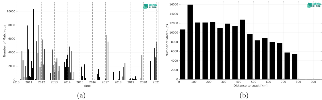
Figure 2: Number of match-ups between TSG (GOSUD-Sailing-ship) and SMOS SSS L2 v700 (ESA) SSS as a function of time (a) and as function of the distance to coast (b) over the SMOS coastal zone (<800km) 60N-60S Pi-MEP region and for the full satellite product period.
