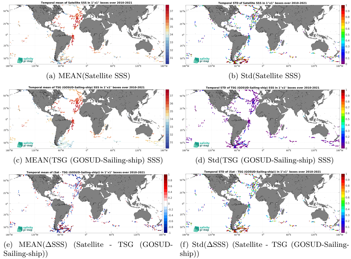
Figure 7: Temporal mean (left) and Std (right) of SSS from SMOS SSS L2 v700 (ESA) (top), TSG (GOSUD-Sailing-ship) (middle), and of \Delta SSS (Satellite - TSG (GOSUD-Sailing-ship)). Only match-up pairs are used to generate these maps.
