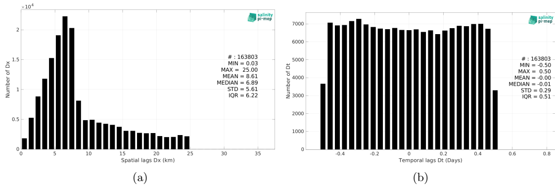
Figure 6: Histograms of the spatial (a) and temporal (b) lags between the location/time of the TSG (GOSUD-Sailing-ship) measurement and the date of the corresponding SMOS SSS L2 v700 (ESA) SSS pixel.
