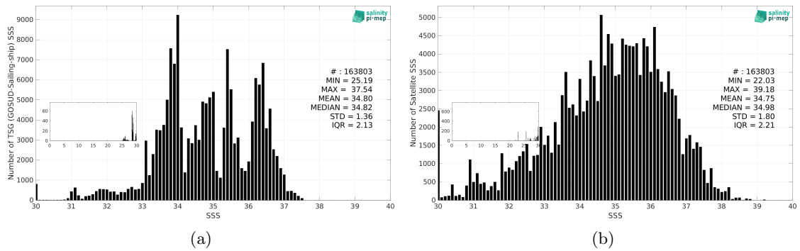
Figure 3: Histograms of SSS from TSG (GOSUD-Sailing-ship) (a) and SMOS SSS L2 v700 (ESA) (b) considering all match-up pairs per bins of 0.1 over the SMOS coastal zone (<800km) 60N-60S Pi-MEP region and for the full satellite product period.
