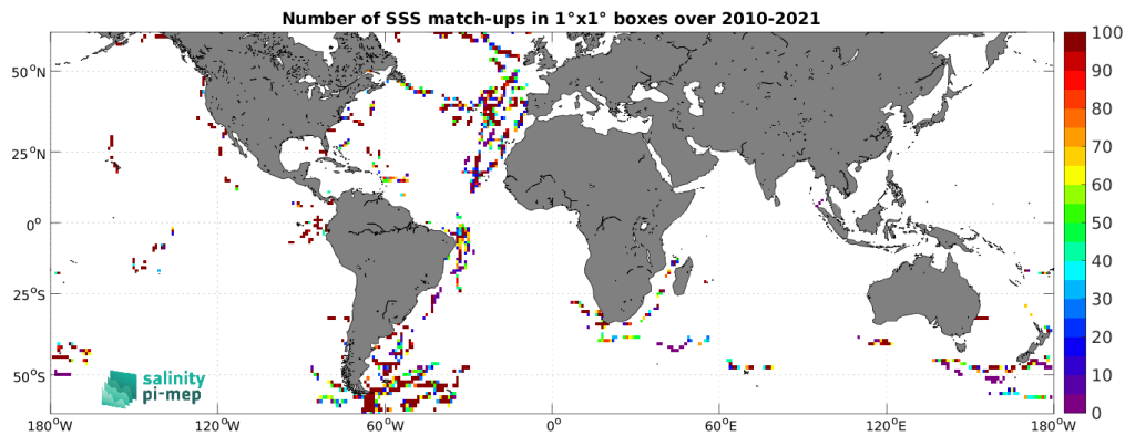
Figure 5: Number of SSS match-ups between TSG (GOSUD-Sailing-ship) SSS and the SMOS SSS L2 v700 (ESA) SSS product for the SMOS coastal zone (<800km) 60N-60S Pi-MEP region over 1^\circ \times 1^\circ boxes and for the full satellite product period.
