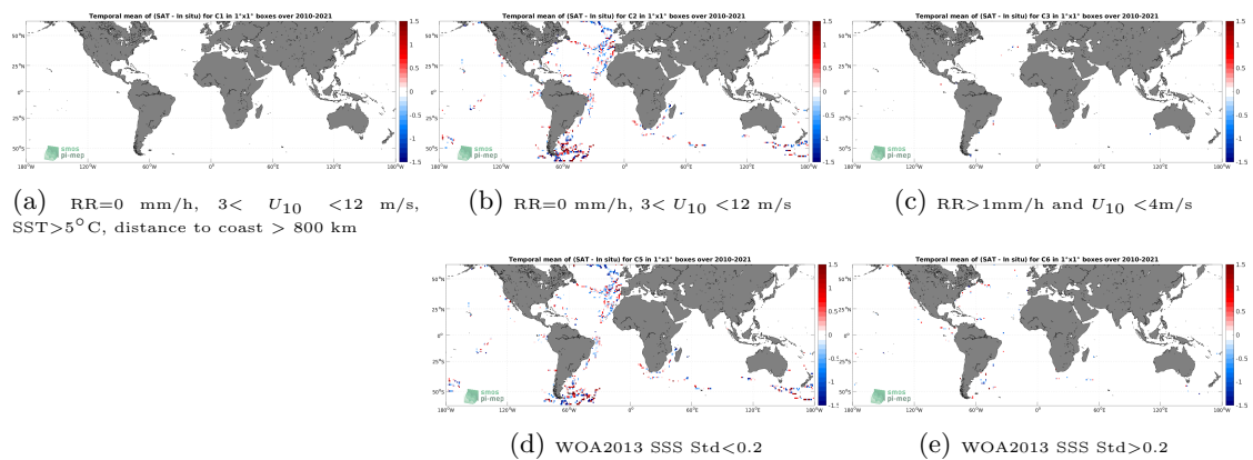
Figure 12: Temporal mean gridded over spatial boxes of size 1^\circ \times 1^\circ of \Delta\text{SSS} (SMOS SSS L2 v700 (ESA) - TSG (GOSUD-Sailing-ship)) for 5 different subdatasets corresponding to:RR=0 mm/h, 3 < U_{10} < 12 m/s, SST > 5^\circ\text{C} , distance to coast > 800 km (a), RR=0 mm/h, 3 < U_{10} < 12 m/s (b), RR > 1 mm/h and U_{10} < 4 m/s (c), WOA2013 SSS Std < 0.2 (d), WOA2013 SSS Std > 0.2 (e).
