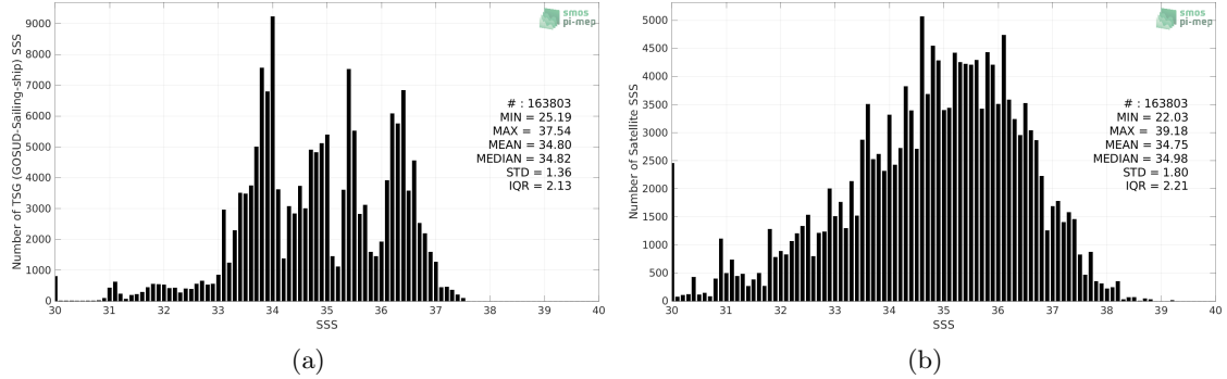
Figure 2: Histograms of SSS from TSG (GOSUD-Sailing-ship) (a) and SMOS SSS L2 v700 (ESA) (b) considering all match-up pairs per bins of 0.1 over the SMOS coastal zone (<800km) 60N-60S Pi-MEP region and for the full satellite product period.
