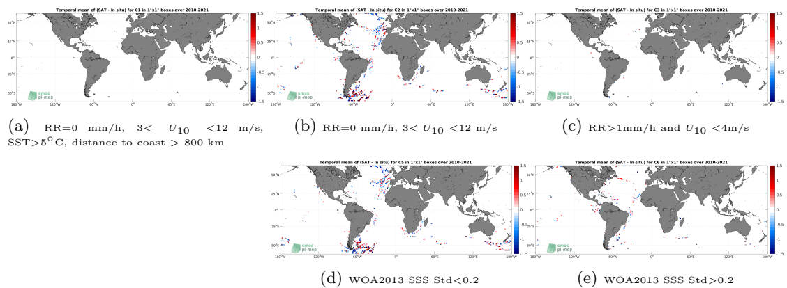
Figure 12: Temporal mean gridded over spatial boxes of size 1^\circ \times 1^\circ of \Delta SSS (SMOS SSS L2 v700 (ESA) - TSG (GOSUD-Sailing-ship)) for 5 different subdatasets corresponding to:RR=0 mm/h, 3 < U_{10} < 12 m/s, SST > 5^\circ\text{C} , distance to coast > 800 km (a), RR=0 mm/h, 3 < U_{10} < 12 m/s (b), RR > 1 mm/h and U_{10} < 4 m/s (c), WOA2013 SSS Std < 0.2 (d), WOA2013 SSS Std > 0.2 (e).
