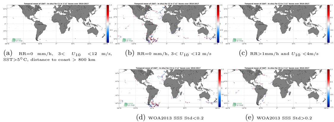
Figure 12: Temporal mean gridded over spatial boxes of size 1^\circ \times 1^\circ of \Delta SSS (SMOS SSS L2 v700 (ESA) - TSG (GOSUD-Sailing-ship)) for 5 different subdatasets corresponding to: RR=0 mm/h, 3 < U_{10} < 12 m/s, SST > 5°C, distance to coast > 800 km (a), RR=0 mm/h, 3 < U_{10} < 12 m/s (b), RR > 1mm/h and U_{10} < 4 m/s (c), WOA2013 SSS Std < 0.2 (d), WOA2013 SSS Std > 0.2 (e).
