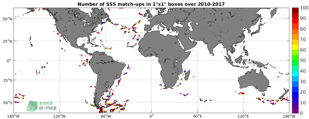
Figure 4: Number of SSS match-ups between TSG (GOSUD-Sailing-ship) SSS and the SMOS SSS L2 v700 (ESA) SSS product for the SMOS coastal zone (<800km) 60N-60S Pi-MEP region over 1^{\circ} \times 1^{\circ} boxes and for the full satellite product period.
