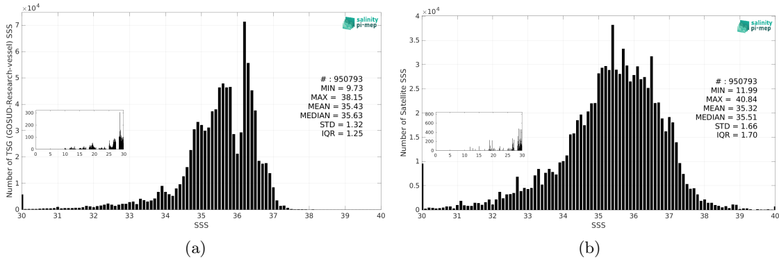
Figure 3: Histograms of SSS from TSG (GOSUD-Research-vessel) (a) and SMOS SSS L2 v700 (ESA) (b) considering all match-up pairs per bins of 0.1 over the SMOS coastal zone (<800km) 60N-60S Pi-MEP region and for the full satellite product period.
