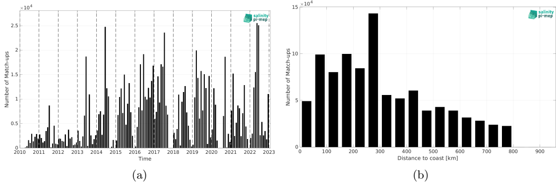
Figure 2: Number of match-ups between TSG (GOSUD-Research-vessel) and SMOS SSS L2 v700 (ESA) SSS as a function of time (a) and as function of the distance to coast (b) over the SMOS coastal zone (<800km) 60N-60S Pi-MEP region and for the full satellite product period.
