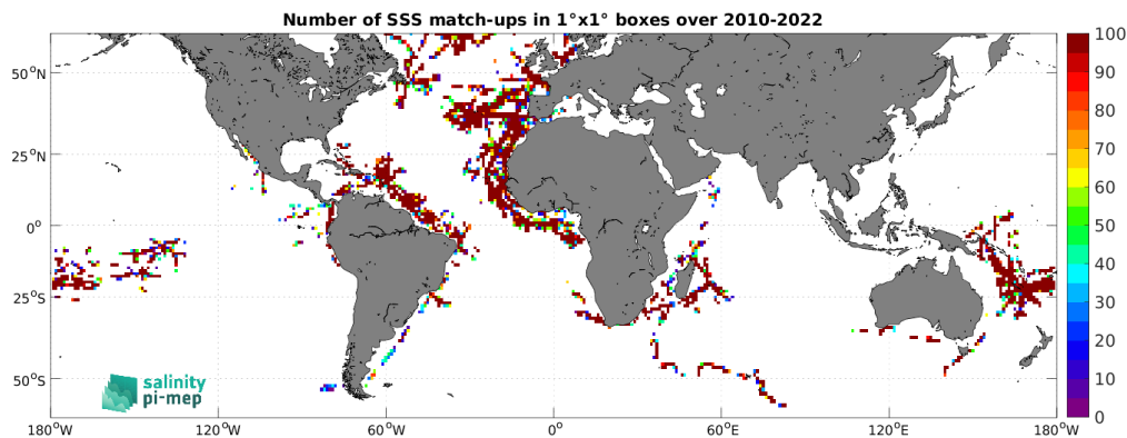
Figure 5: Number of SSS match-ups between TSG (GOSUD-Research-vessel) SSS and the SMOS SSS L2 v700 (ESA) SSS product for the SMOS coastal zone (<800km) 60N-60S Pi-MEP region over 1^\circ \times 1^\circ boxes and for the full satellite product period.
