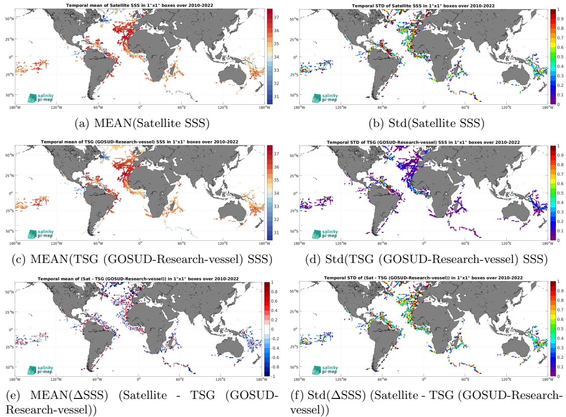
Figure 7: Temporal mean (left) and Std (right) of SSS from SMOS SSS L2 v700 (ESA) (top), TSG (GOSUD-Research-vessel) (middle), and of \Delta SSS (Satellite - TSG (GOSUD-Research-vessel)). Only match-up pairs are used to generate these maps.
