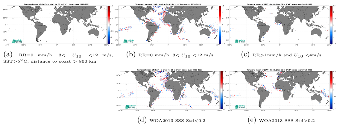
Figure 14: Temporal mean gridded over spatial boxes of size 1^\circ \times 1^\circ of \Delta SSS (SMOS SSS L2 v700 (ESA) - TSG (GOSUD-Research-vessel)) for 5 different subdatasets corresponding to:RR=0 mm/h, 3 < U_{10} < 12 m/s, SST >5^\circ\text{C} , distance to coast > 800 km (a), RR=0 mm/h, 3 < U_{10} < 12 m/s (b), RR >1 mm/h and U_{10} < 4 m/s (c), WOA2013 SSS Std <0.2 (d), WOA2013 SSS Std >0.2 (e).
