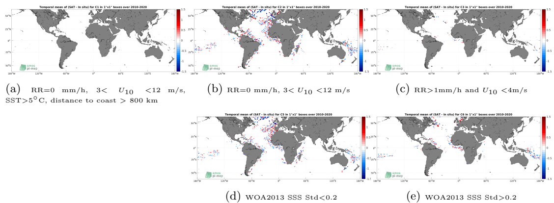
Figure 12: Temporal mean gridded over spatial boxes of size 1^\circ \times 1^\circ of \Delta SSS (SMOS SSS L2 v700 (ESA) - TSG (GOSUD-Research-vessel)) for 5 different subdatasets corresponding to:RR=0 mm/h, 3 < U_{10} < 12 m/s, SST >5^\circ\text{C} , distance to coast > 800 km (a), RR=0 mm/h, 3 < U_{10} < 12 m/s (b), RR >1 mm/h and U_{10} < 4 m/s (c), WOA2013 SSS Std <0.2 (d), WOA2013 SSS Std >0.2 (e).
