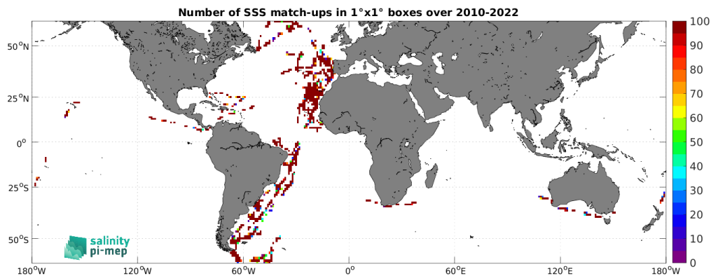
Figure 5: Number of SSS match-ups between TSG (CSIC-UTM) SSS and the SMOS SSS L2 v700 (ESA) SSS product for the SMOS coastal zone (<800km) 60N-60S Pi-MEP region over 1^\circ \times 1^\circ boxes and for the full satellite product period.
