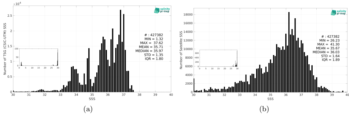
Figure 3: Histograms of SSS from TSG (CSIC-UTM) (a) and SMOS SSS L2 v700 (ESA) (b) considering all match-up pairs per bins of 0.1 over the SMOS coastal zone (<800km) 60N-60S Pi-MEP region and for the full satellite product period.
