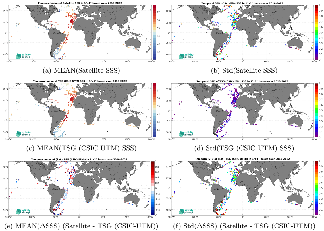
Figure 7: Temporal mean (left) and Std (right) of SSS from SMOS SSS L2 v700 (ESA) (top), TSG (CSIC-UTM) (middle), and of \Delta SSS (Satellite - TSG (CSIC-UTM)). Only match-up pairs are used to generate these maps.
