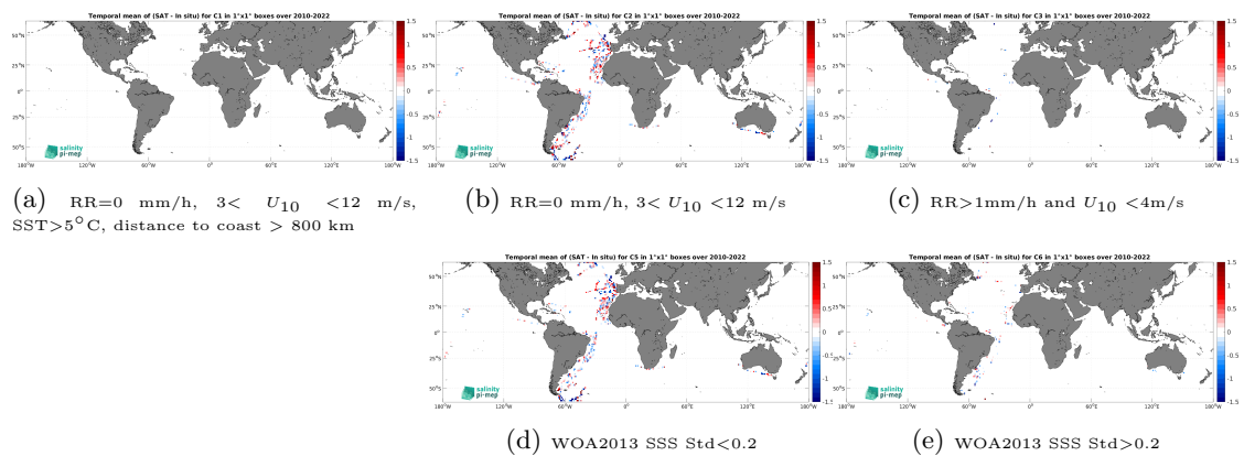
Figure 14: Temporal mean gridded over spatial boxes of size 1^\circ \times 1^\circ of \Delta\text{SSS} (SMOS SSS L2 v700 (ESA) - TSG (CSIC-UTM)) for 5 different subdatasets corresponding to:RR=0 mm/h, 3 < U_{10} < 12 m/s, SST>5°C, distance to coast > 800 km (a), RR=0 mm/h, 3 < U_{10} < 12 m/s (b), RR>1mm/h and U_{10} < 4 m/s (c), WOA2013 SSS Std<0.2 (d), WOA2013 SSS Std>0.2 (e).
