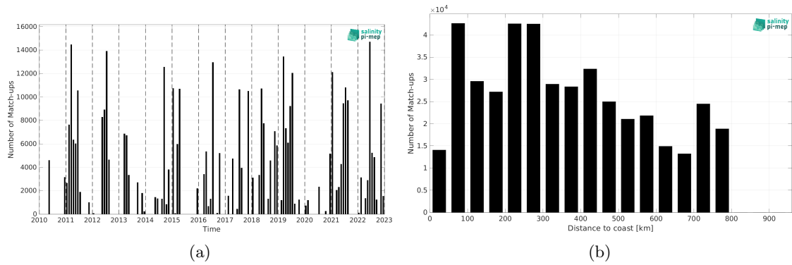
Figure 2: Number of match-ups between TSG (CSIC-UTM) and SMOS SSS L2 v700 (ESA) SSS as a function of time (a) and as function of the distance to coast (b) over the SMOS coastal zone (<800km) 60N-60S Pi-MEP region and for the full satellite product period.
