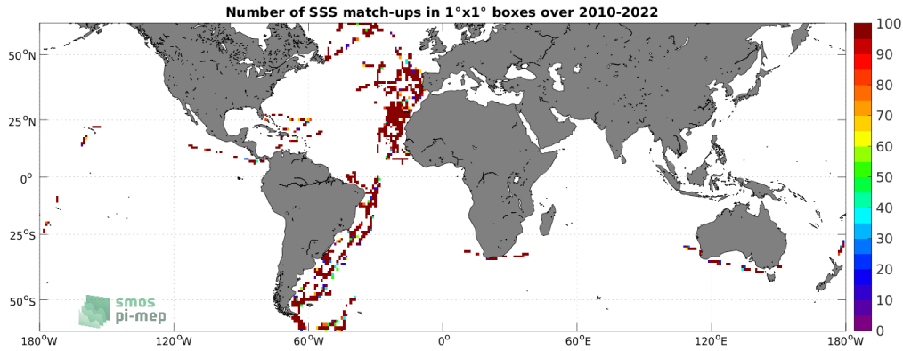
Figure 4: Number of SSS match-ups between TSG (CSIC-UTM) SSS and the SMOS SSS L2 v700 (ESA) SSS product for the SMOS coastal zone (<800km) 60N-60S Pi-MEP region over 1^\circ \times 1^\circ boxes and for the full satellite product period.
