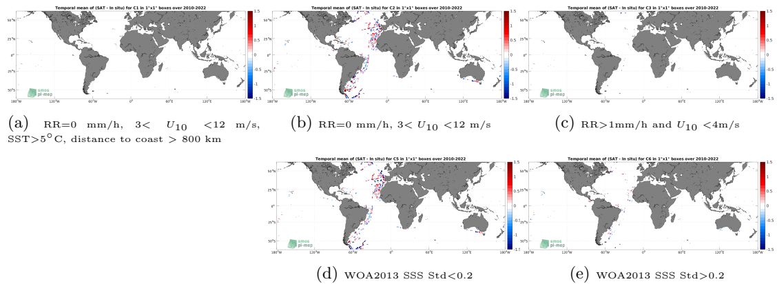
Figure 12: Temporal mean gridded over spatial boxes of size 1^\circ \times 1^\circ of \Delta SSS (SMOS SSS L2 v700 (ESA) - TSG (CSIC-UTM)) for 5 different subdatasets corresponding to:RR=0 mm/h, 3 < U_{10} < 12 m/s, SST >5^\circ\text{C} , distance to coast > 800 km (a), RR=0 mm/h, 3 < U_{10} < 12 m/s (b), RR >1 mm/h and U_{10} < 4 m/s (c), WOA2013 SSS Std <0.2 (d), WOA2013 SSS Std >0.2 (e).
