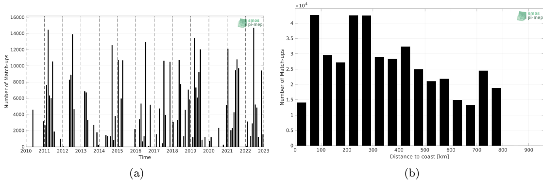
Figure 1: Number of match-ups between TSG (CSIC-UTM) and SMOS SSS L2 v700 (ESA) SSS as a function of time (a) and as function of the distance to coast (b) over the SMOS coastal zone (<800km) 60N-60S Pi-MEP region and for the full satellite product period.
