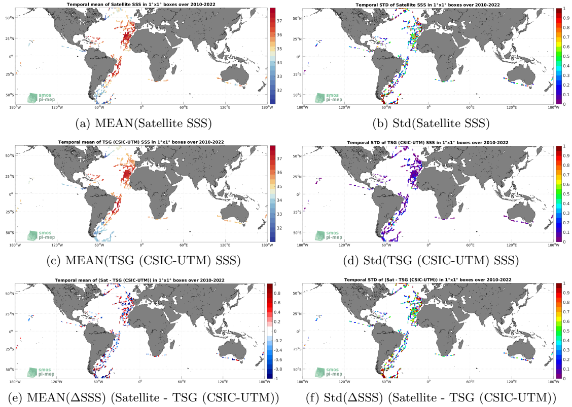
Figure 6: Temporal mean (left) and Std (right) of SSS from SMOS SSS L2 v700 (ESA) (top), TSG (CSIC-UTM) (middle), and of \Delta SSS (Satellite - TSG (CSIC-UTM)). Only match-up pairs are used to generate these maps.
