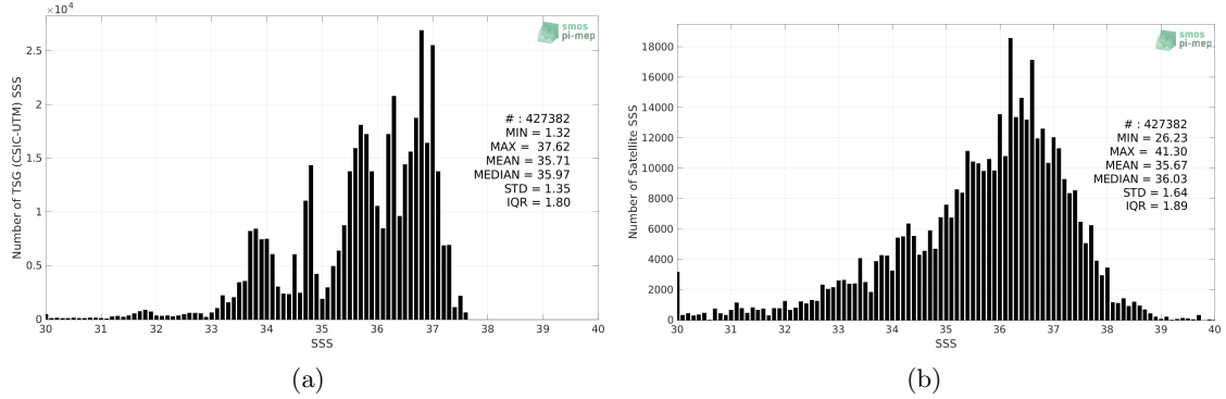
Figure 2: Histograms of SSS from TSG (CSIC-UTM) (a) and SMOS SSS L2 v700 (ESA) (b) considering all match-up pairs per bins of 0.1 over the SMOS coastal zone (<800km) 60N-60S Pi-MEP region and for the full satellite product period.
