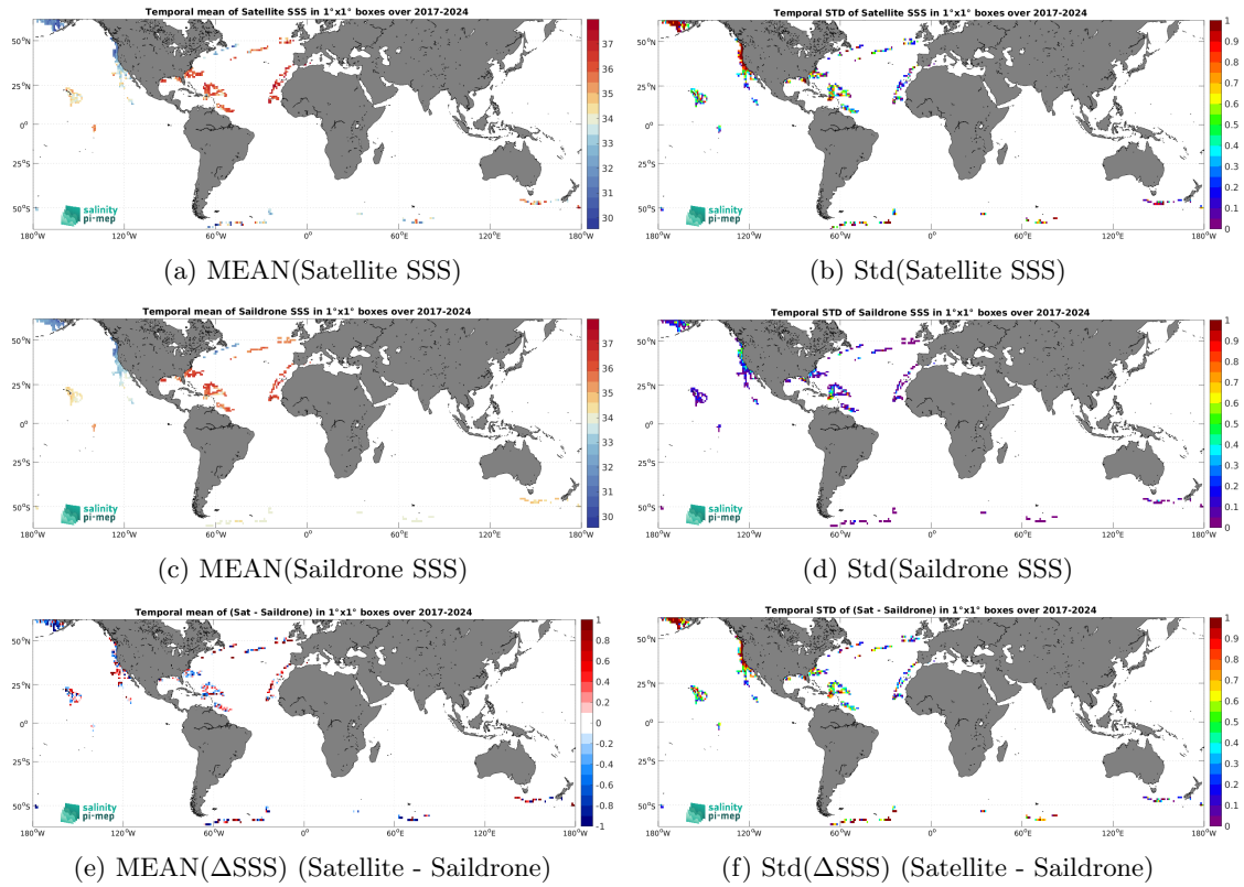
Figure 7: Temporal mean (left) and Std (right) of SSS from SMOS SSS L2 v700 (ESA) (top), Saildrone (middle), and of \Delta SSS (Satellite - Saildrone). Only match-up pairs are used to generate these maps.
