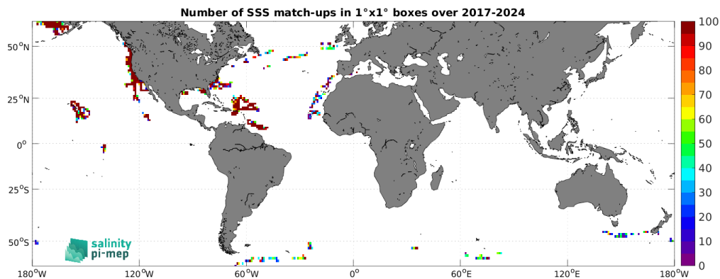
Figure 5: Number of SSS match-ups between Saildrone SSS and the SMOS SSS L2 v700 (ESA) SSS product for the SMOS coastal zone (<800km) 60N-60S Pi-MEP region over 1^\circ \times 1^\circ boxes and for the full satellite product period.
