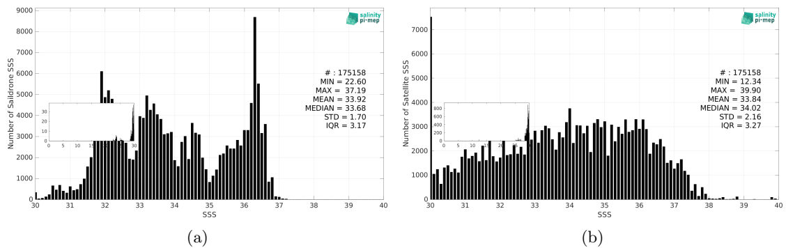
Figure 3: Histograms of SSS from Sairdrone (a) and SMOS SSS L2 v700 (ESA) (b) considering all match-up pairs per bins of 0.1 over the SMOS coastal zone (<800km) 60N-60S Pi-MEP region and for the full satellite product period.
