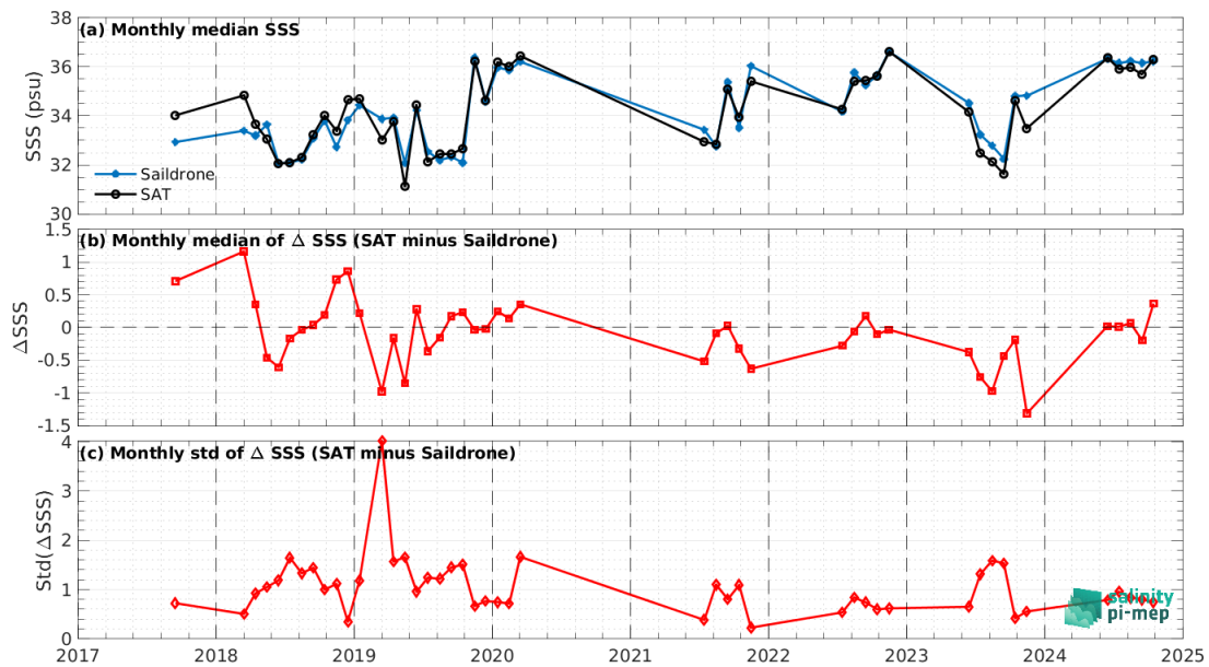
Figure 8: Time series of the monthly median SSS (top), median of \Delta SSS (Satellite - Sairdron) and Std of \Delta SSS (Satellite - Sairdron) over the SMOS coastal zone ( <800\text{km} ) 60\text{N} - 60\text{S} Pi-MEP region considering all match-ups collected by the Pi-MEP.
