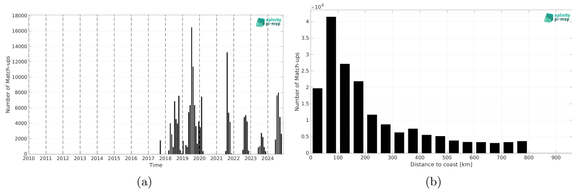
Figure 2: Number of match-ups between Sairdrone and SMOS SSS L2 v700 (ESA) SSS as a function of time (a) and as function of the distance to coast (b) over the SMOS coastal zone (<800km) 60N-60S Pi-MEP region and for the full satellite product period.
