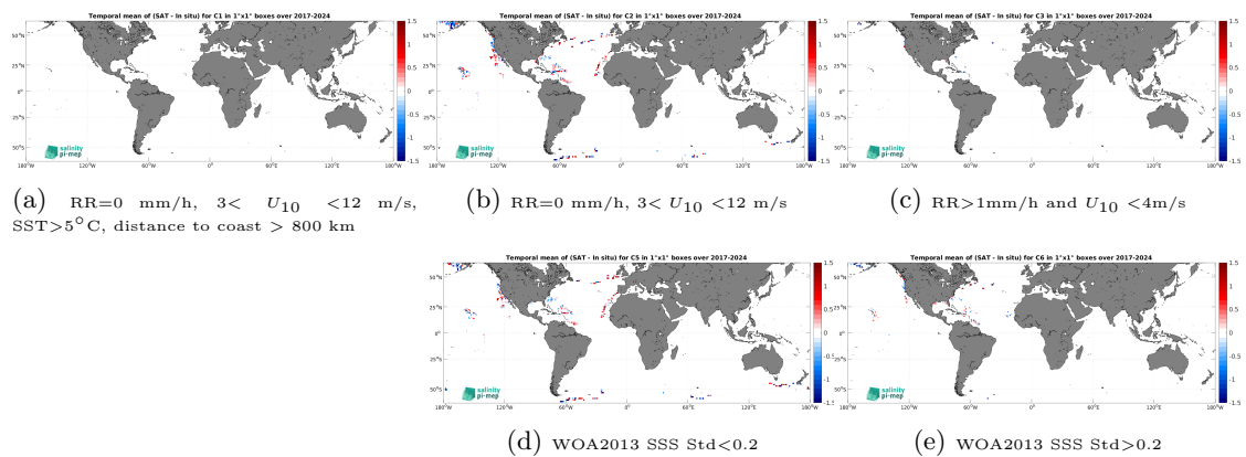
Figure 14: Temporal mean gridded over spatial boxes of size 1^\circ \times 1^\circ of \Delta\text{SSS} (SMOS SSS L2 v700 (ESA) - Sairdron) for 5 different subdatasets corresponding to:RR=0 mm/h, 3 < U_{10} < 12 m/s, SST > 5°C, distance to coast > 800 km (a), RR=0 mm/h, 3 < U_{10} < 12 m/s (b), RR > 1mm/h and U_{10} < 4 m/s (c), WOA2013 SSS Std < 0.2 (d), WOA2013 SSS Std > 0.2 (e).
