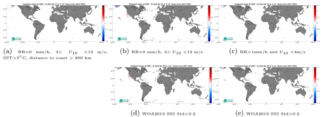
Figure 14: Temporal mean gridded over spatial boxes of size 1^\circ \times 1^\circ of \Delta\text{SSS} (SMOS SSS L2 v700 (ESA) - Sailyrone) for 5 different subdatasets corresponding to: RR=0 mm/h, 3 < U_{10} < 12 m/s, SST > 5°C, distance to coast > 800 km (a), RR=0 mm/h, 3 < U_{10} < 12 m/s (b), RR > 1mm/h and U_{10} < 4 m/s (c), WOA2013 SSS Std < 0.2 (d), WOA2013 SSS Std > 0.2 (e).
