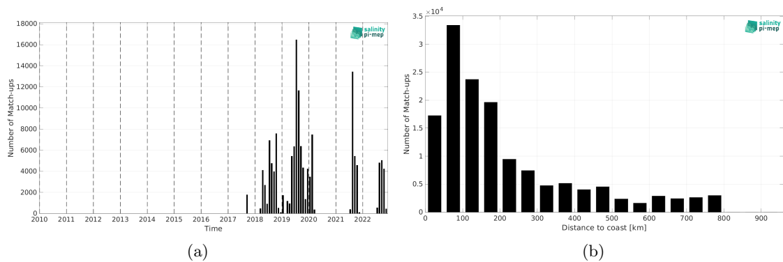
Figure 1: Number of match-ups between Sairdrone and SMOS SSS L2 v700 (ESA) SSS as a function of time (a) and as function of the distance to coast (b) over the SMOS coastal zone (<800km) 60N-60S Pi-MEP region and for the full satellite product period.
