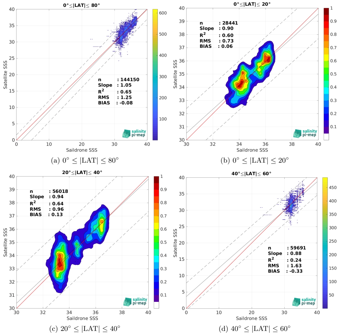
Figure 9: Contour maps of the concentration of SMOS SSS L2 v700 (ESA) SSS (y-axis) versus Saildrone SSS (x-axis) at match-up pairs for different latitude bands. For each plot, the red line shows x=y . The black thin and dashed lines indicate a linear fit through the data cloud and the \pm 95\% confidence levels, respectively. The number match-up pairs n , the slope and R^2 coefficient of the linear fit, the root mean square (RMS) and the mean bias between satellite and in situ data are indicated for each latitude band in each plots.
