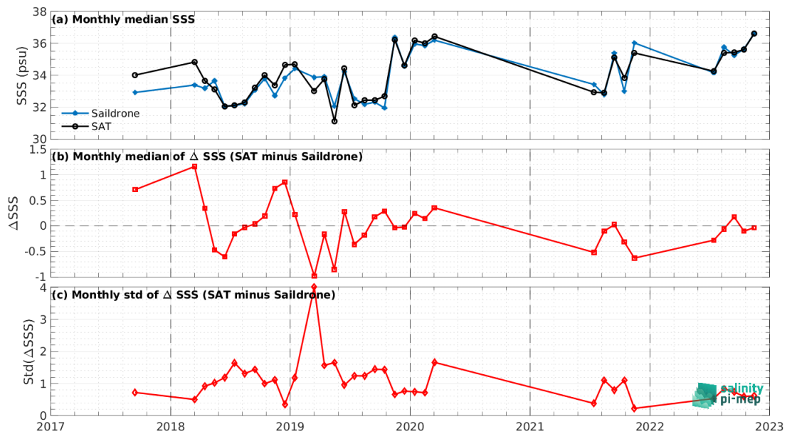
Figure 7: Time series of the monthly median SSS (top), median of \Delta SSS (Satellite - Sairdrone) and Std of \Delta SSS (Satellite - Sairdrone) over the SMOS coastal zone (<800km) 60N-60S Pi-MEP region considering all match-ups collected by the Pi-MEP.
