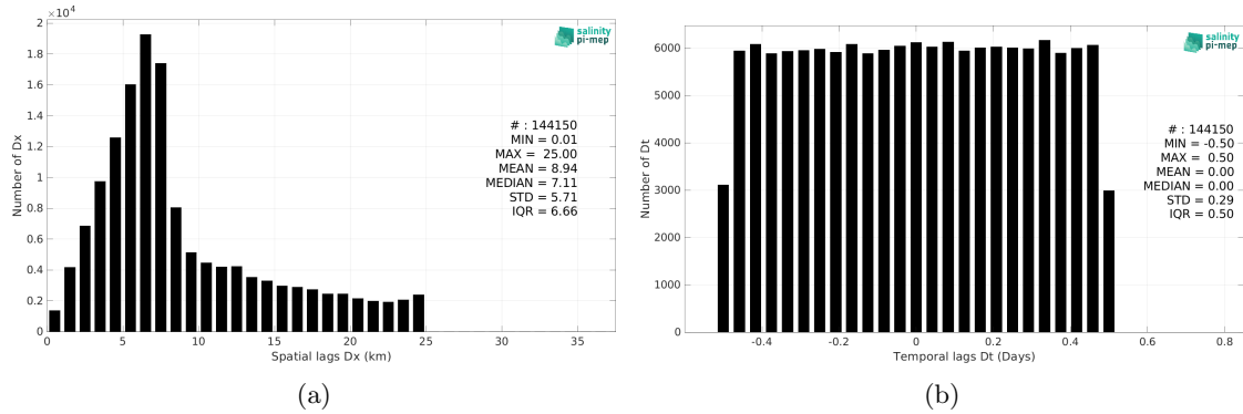
Figure 5: Histograms of the spatial (a) and temporal (b) lags between the location/time of the Saildrone measurement and the date of the corresponding SMOS SSS L2 v700 (ESA) SSS pixel.
