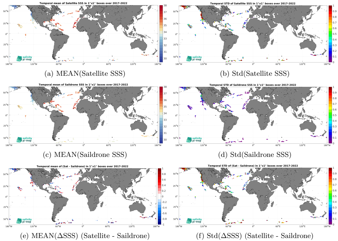
Figure 6: Temporal mean (left) and Std (right) of SSS from SMOS SSS L2 v700 (ESA) (top), Saildrone (middle), and of \Delta SSS (Satellite - Saildrone). Only match-up pairs are used to generate these maps.
