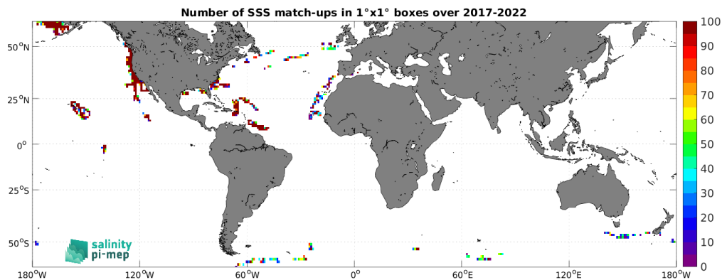
Figure 4: Number of SSS match-ups between Saildrone SSS and the SMOS SSS L2 v700 (ESA) SSS product for the SMOS coastal zone (<800km) 60N-60S Pi-MEP region over 1^\circ \times 1^\circ boxes and for the full satellite product period.
