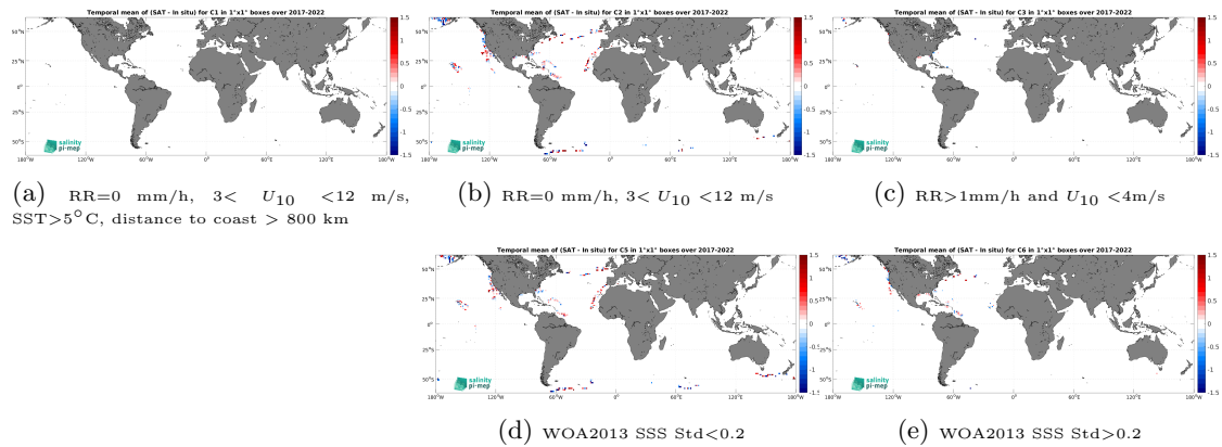
Figure 12: Temporal mean gridded over spatial boxes of size 1^\circ \times 1^\circ of \Delta\text{SSS} (SMOS SSS L2 v700 (ESA) - Saldrone) for 5 different subdatasets corresponding to:RR=0 mm/h, 3 < U_{10} < 12 m/s, SST >5^\circ\text{C} , distance to coast > 800 km (a), RR=0 mm/h, 3 < U_{10} < 12 m/s (b), RR >1 mm/h and U_{10} < 4 m/s (c), WOA2013 SSS Std <0.2 (d), WOA2013 SSS Std >0.2 (e).
