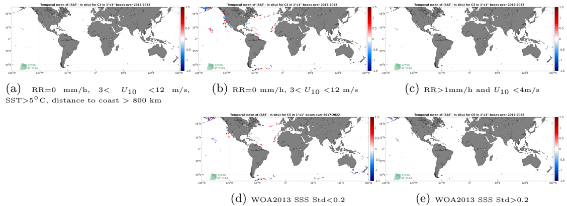
Figure 12: Temporal mean gridded over spatial boxes of size 1^\circ \times 1^\circ of \Delta SSS (SMOS SSS L2 v700 (ESA) - Saldrone) for 5 different subdatasets corresponding to:RR=0 mm/h, 3 < U_{10} < 12 m/s, SST >5^\circ\text{C} , distance to coast > 800 km (a), RR=0 mm/h, 3 < U_{10} < 12 m/s (b), RR >1 mm/h and U_{10} < 4 m/s (c), WOA2013 SSS Std <0.2 (d), WOA2013 SSS Std >0.2 (e).
