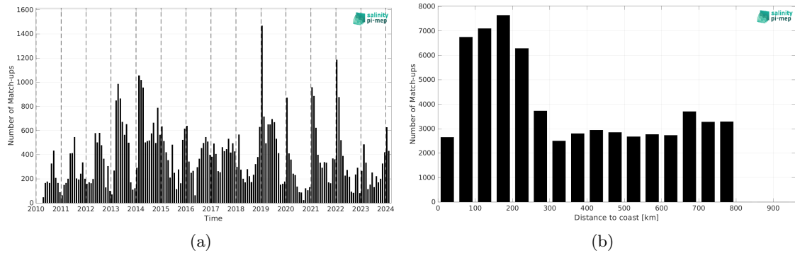
Figure 2: Number of match-ups between Marine mammals and SMOS SSS L2 v700 (ESA) SSS as a function of time (a) and as function of the distance to coast (b) over the SMOS coastal zone (<800km) 60N-60S Pi-MEP region and for the full satellite product period.
