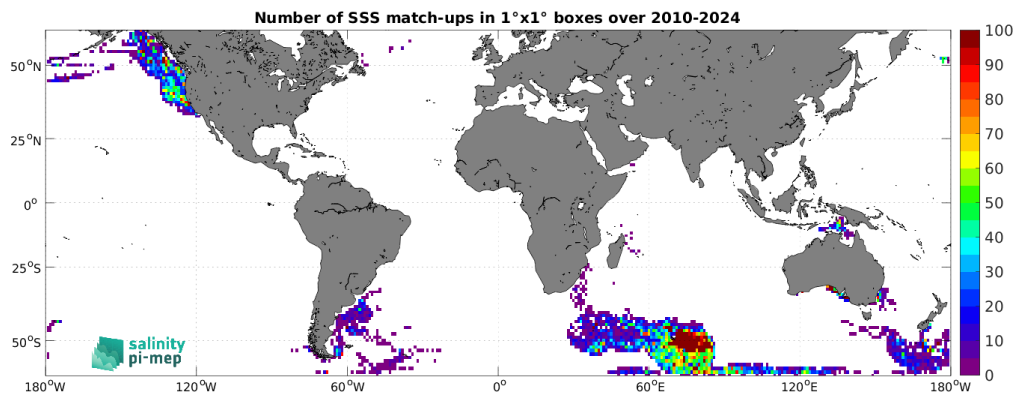
Figure 5: Number of SSS match-ups between Marine mammals SSS and the SMOS SSS L2 v700 (ESA) SSS product for the SMOS coastal zone (<800km) 60N-60S Pi-MEP region over 1^\circ \times 1^\circ boxes and for the full satellite product period.
