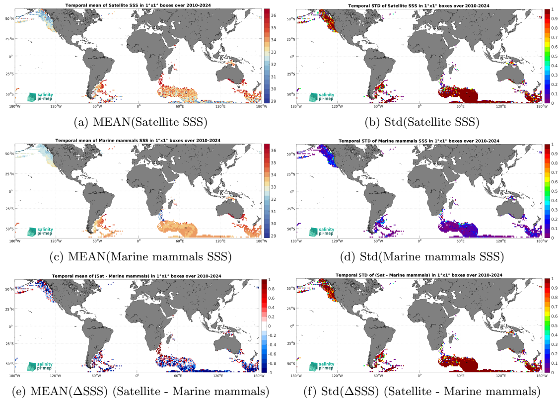
Figure 7: Temporal mean (left) and Std (right) of SSS from SMOS SSS L2 v700 (ESA) (top), Marine mammals (middle), and of \Delta SSS (Satellite - Marine mammals). Only match-up pairs are used to generate these maps.
