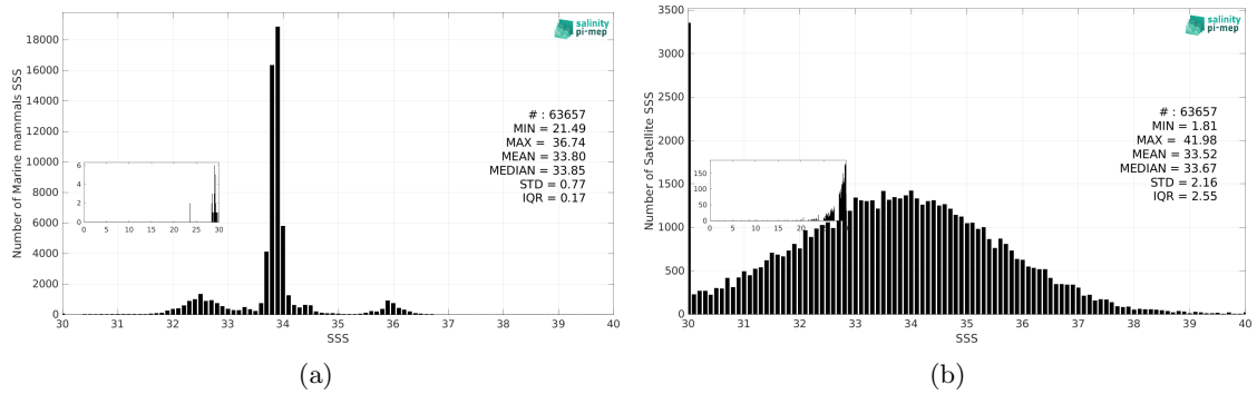
Figure 3: Histograms of SSS from Marine mammals (a) and SMOS SSS L2 v700 (ESA) (b) considering all match-up pairs per bins of 0.1 over the SMOS coastal zone (<800km) 60N-60S Pi-MEP region and for the full satellite product period.
