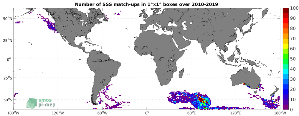
Figure 4: Number of SSS match-ups between Marine mammals SSS and the SMOS SSS L2 v700 (ESA) SSS product for the SMOS coastal zone (<800km) 60N-60S Pi-MEP region over 1°×1° boxes and for the full satellite product period.
