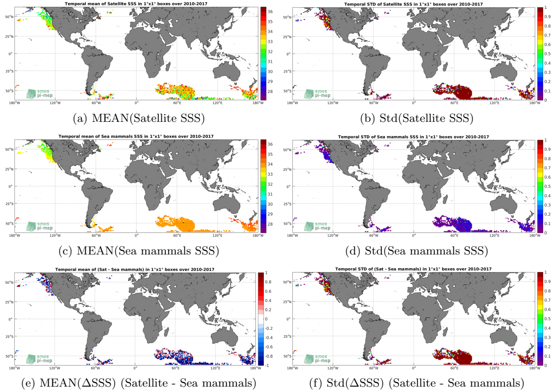
Figure 6: Temporal mean (left) and Std (right) of SSS from SMOS SSS L2 v700 (ESA) (top), Sea mammals (middle), and of \Delta SSS (Satellite - Sea mammals). Only match-up pairs are used to generate these maps.
