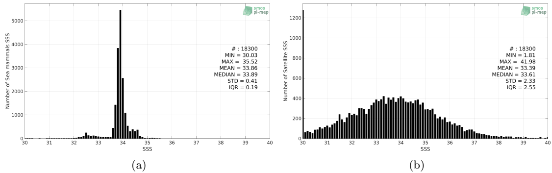
Figure 2: Histograms of SSS from Sea mammals (a) and SMOS SSS L2 v700 (ESA) (b) considering all match-up pairs per bins of 0.1 over the SMOS coastal zone (<800km) 60N-60S Pi-MEP region and for the full satellite product period.
