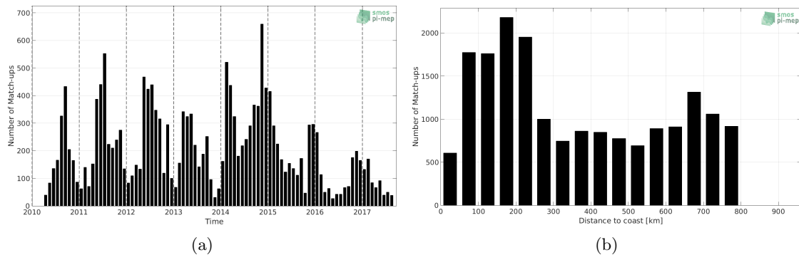
Figure 1: Number of match-ups between Sea mammals and SMOS SSS L2 v700 (ESA) SSS as a function of time (a) and as function of the distance to coast (b) over the SMOS coastal zone (<800km) 60N-60S Pi-MEP region and for the full satellite product period.
