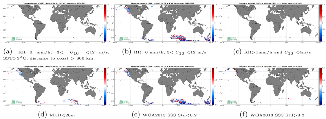
Figure 12: Temporal mean gridded over spatial boxes of size 1^\circ \times 1^\circ of \Delta SSS (SMOS SSS L2 v700 (ESA) - Sea mammals) for 6 different subdatasets corresponding to:RR=0 mm/h, 3 < U_{10} < 12 m/s, SST >5^\circ\text{C} , distance to coast > 800 km (a), RR=0 mm/h, 3 < U_{10} < 12 m/s (b), RR >1 mm/h and U_{10} < 4 m/s (c),MLD <20 m (d),WOA2013 SSS Std <0.2 (e),WOA2013 SSS Std >0.2 (f).
