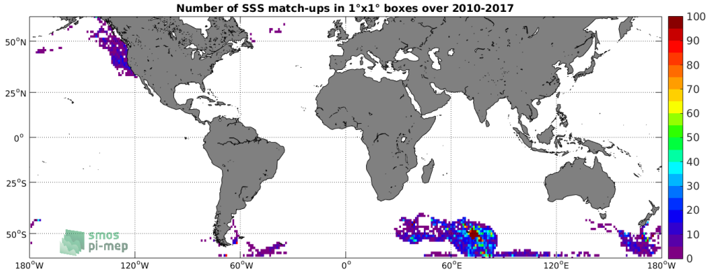
Figure 4: Number of SSS match-ups between Sea mammals SSS and the SMOS SSS L2 v700 (ESA) SSS product for the SMOS coastal zone (<800km) 60N-60S Pi-MEP region over 1^\circ \times 1^\circ boxes and for the full satellite product period.
