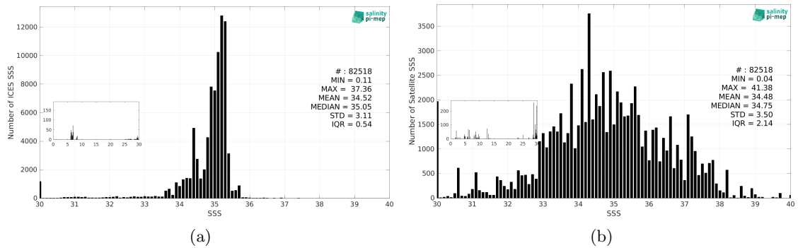
Figure 3: Histograms of SSS from ICES (a) and SMOS SSS L2 v700 (ESA) (b) considering all match-up pairs per bins of 0.1 over the SMOS coastal zone (<800km) 60N-60S Pi-MEP region and for the full satellite product period.
