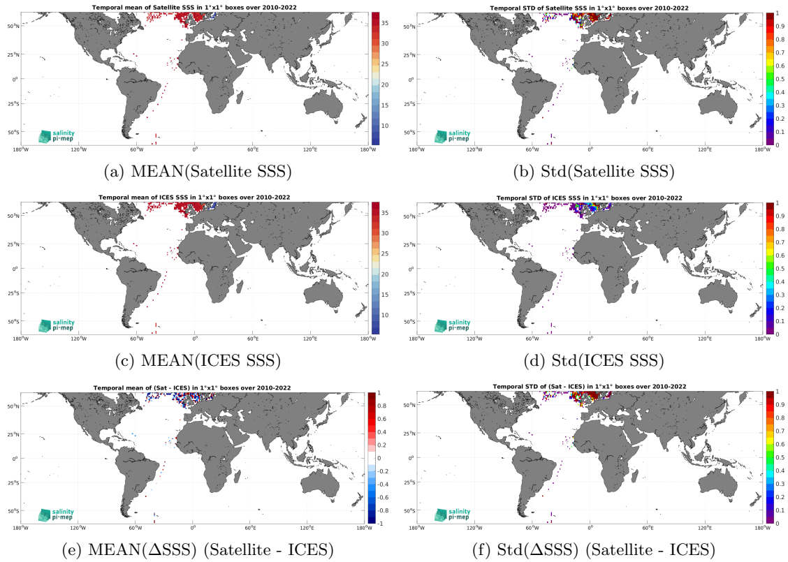
Figure 7: Temporal mean (left) and Std (right) of SSS from SMOS SSS L2 v700 (ESA) (top), ICES (middle), and of \Delta SSS (Satellite - ICES). Only match-up pairs are used to generate these maps.
