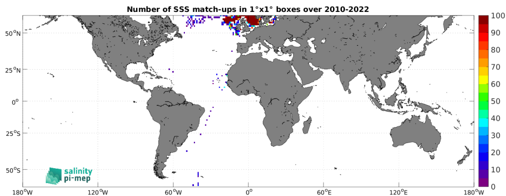
Figure 5: Number of SSS match-ups between ICES SSS and the SMOS SSS L2 v700 (ESA) SSS product for the SMOS coastal zone (<800km) 60N-60S Pi-MEP region over 1^\circ \times 1^\circ boxes and for the full satellite product period.
