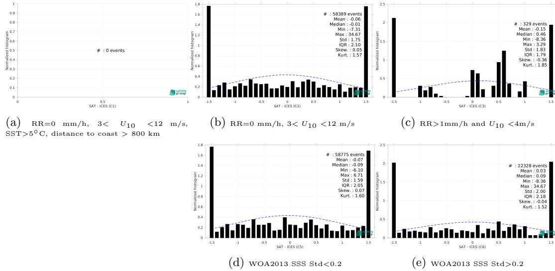
Figure 15: Normalized histogram of \Delta SSS (SMOS SSS L2 v700 (ESA) - ICES) for 5 different subdatasets corresponding to: RR=0 mm/h, 3 < U_{10} < 12 m/s, SST > 5°C, distance to coast > 800 km (a), RR=0 mm/h, 3 < U_{10} < 12 m/s (b), RR > 1mm/h and U_{10} < 4 m/s (c), WOA2013 SSS Std < 0.2 (d), WOA2013 SSS Std > 0.2 (e).
