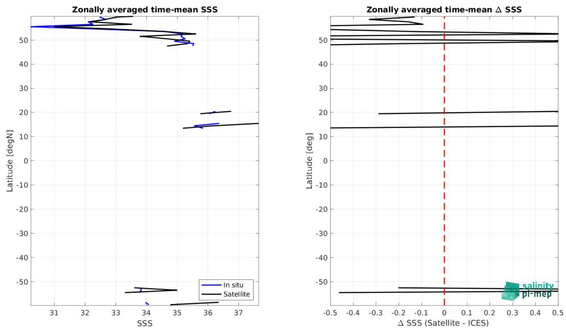
Figure 9: Left panel: Zonal mean SSS from SMOS SSS L2 v700 (ESA) satellite product (black) and from ICES (blue). Right panel: Zonal mean of \Delta SSS (Satellite - ICES) for all the collected Pi-MEP match-up pairs estimated over the full satellite product period.
