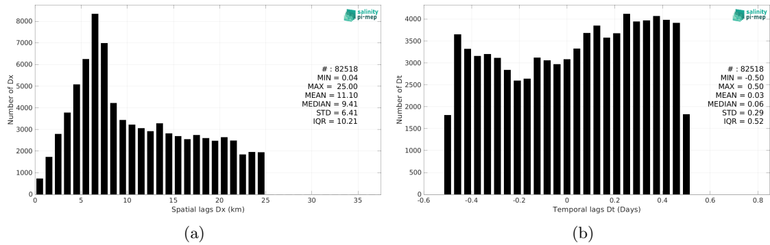
Figure 6: Histograms of the spatial (a) and temporal (b) lags between the location/time of the ICES measurement and the date of the corresponding SMOS SSS L2 v700 (ESA) SSS pixel.
