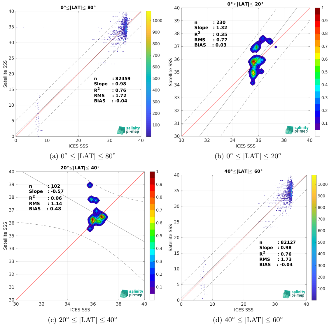
Figure 10: Contour maps of the concentration of SMOS SSS L2 v700 (ESA) SSS (y-axis) versus ICES SSS (x-axis) at match-up pairs for different latitude bands. For each plot, the red line shows x=y . The black thin and dashed lines indicate a linear fit through the data cloud and the \pm 95\% confidence levels, respectively. The number match-up pairs n , the slope and R^2 coefficient of the linear fit, the root mean square (RMS) and the mean bias between satellite and in situ data are indicated for each latitude band in each plots.
