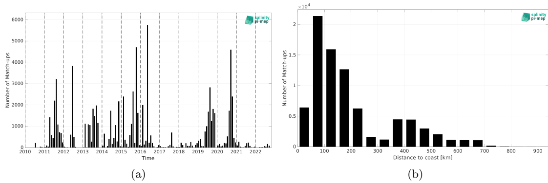
Figure 2: Number of match-ups between ICES and SMOS SSS L2 v700 (ESA) SSS as a function of time (a) and as function of the distance to coast (b) over the SMOS coastal zone (<800km) 60N-60S Pi-MEP region and for the full satellite product period.
