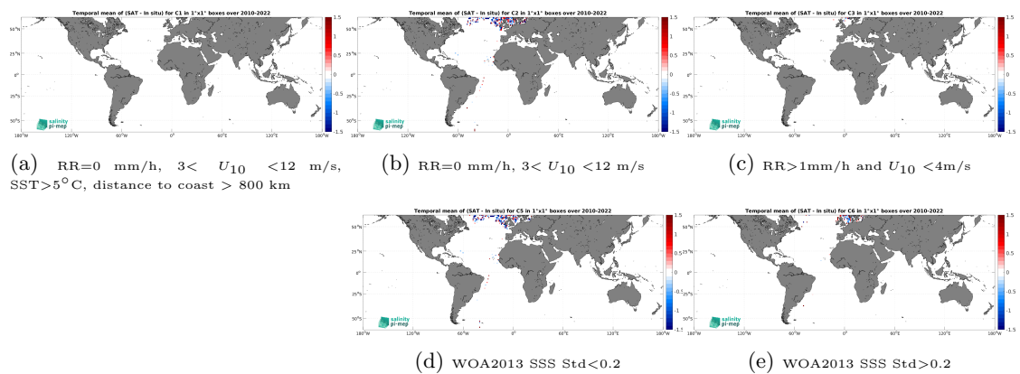
Figure 14: Temporal mean gridded over spatial boxes of size 1^\circ \times 1^\circ of \Delta\text{SSS} (SMOS SSS L2 v700 (ESA) - ICES) for 5 different subdatasets corresponding to: RR=0 mm/h, 3 < U_{10} < 12 m/s, SST > 5°C, distance to coast > 800 km (a), RR=0 mm/h, 3 < U_{10} < 12 m/s (b), RR > 1mm/h and U_{10} < 4 m/s (c), WOA2013 SSS Std < 0.2 (d), WOA2013 SSS Std > 0.2 (e).
