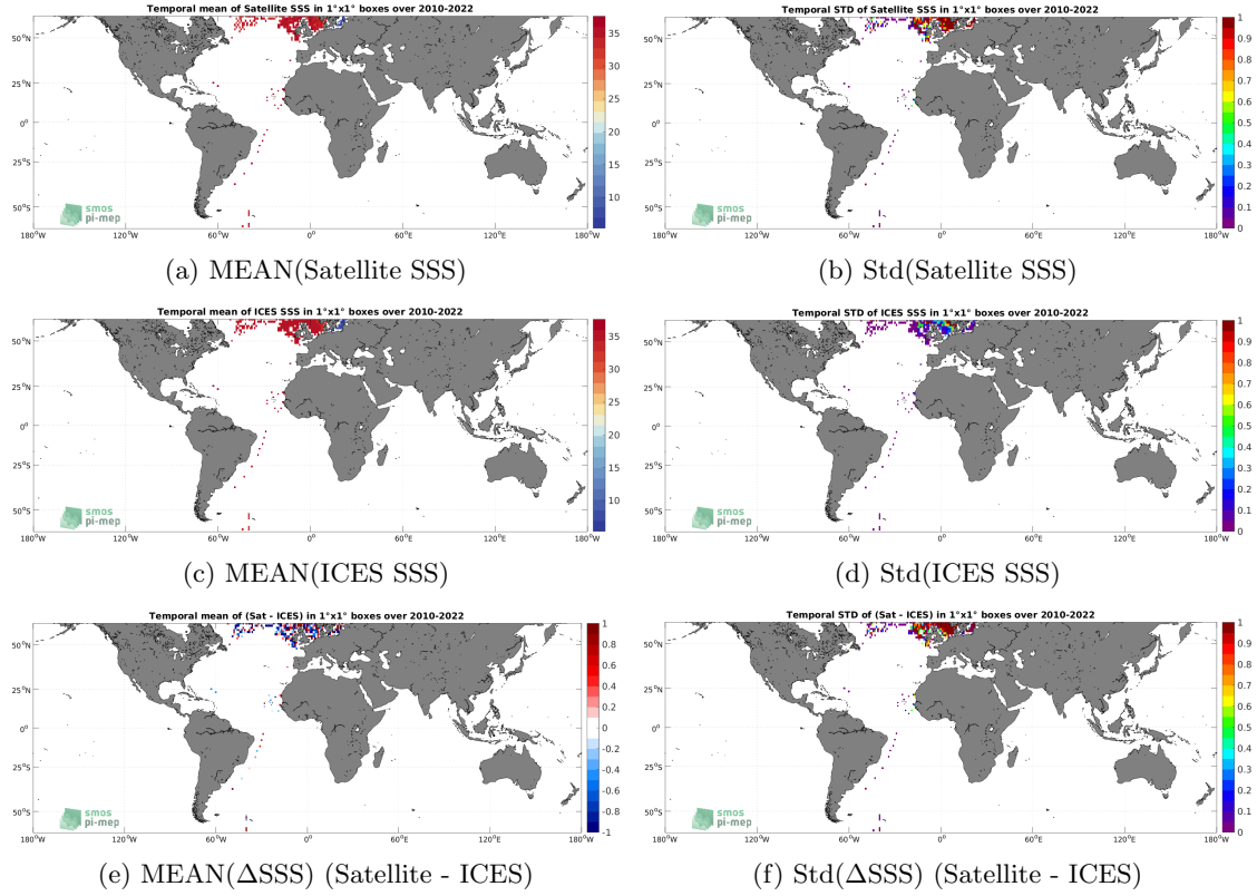
Figure 6: Temporal mean (left) and Std (right) of SSS from SMOS SSS L2 v700 (ESA) (top), ICES (middle), and of \Delta SSS (Satellite - ICES). Only match-up pairs are used to generate these maps.
