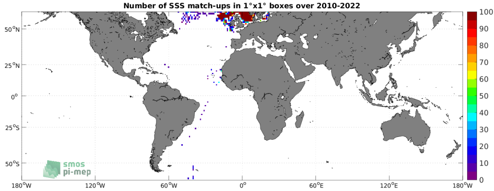
Figure 4: Number of SSS match-ups between ICES SSS and the SMOS SSS L2 v700 (ESA) SSS product for the SMOS coastal zone (<800km) 60N-60S Pi-MEP region over 1^\circ \times 1^\circ boxes and for the full satellite product period.
