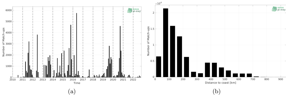
Figure 1: Number of match-ups between ICES and SMOS SSS L2 v700 (ESA) SSS as a function of time (a) and as function of the distance to coast (b) over the SMOS coastal zone (<800km) 60N-60S Pi-MEP region and for the full satellite product period.
