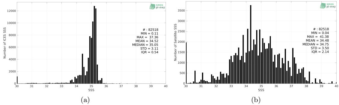
Figure 2: Histograms of SSS from ICES (a) and SMOS SSS L2 v700 (ESA) (b) considering all match-up pairs per bins of 0.1 over the SMOS coastal zone (<800km) 60N-60S Pi-MEP region and for the full satellite product period.
