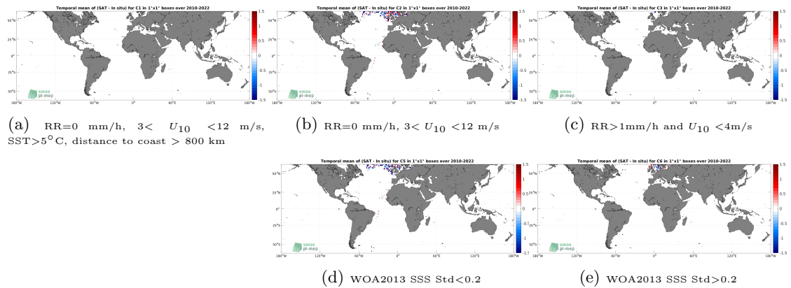
Figure 12: Temporal mean gridded over spatial boxes of size 1^\circ \times 1^\circ of \Delta SSS (SMOS SSS L2 v700 (ESA) - ICES) for 5 different subdatasets corresponding to:RR=0 mm/h, 3 < U_{10} < 12 m/s, SST >5^\circ\text{C} , distance to coast > 800 km (a), RR=0 mm/h, 3 < U_{10} < 12 m/s (b), RR >1 mm/h and U_{10} < 4 m/s (c), WOA2013 SSS Std <0.2 (d), WOA2013 SSS Std >0.2 (e).
