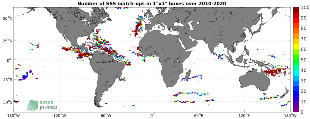
Figure 3: Number of SSS match-ups between Surface drifters SSS and the SMOS SSS L2 v700 (ESA) SSS product for the SMOS coastal zone ( <800\text{km} ) 60N-60S Pi-MEP region over 1^\circ \times 1^\circ boxes and for the full satellite product period.
