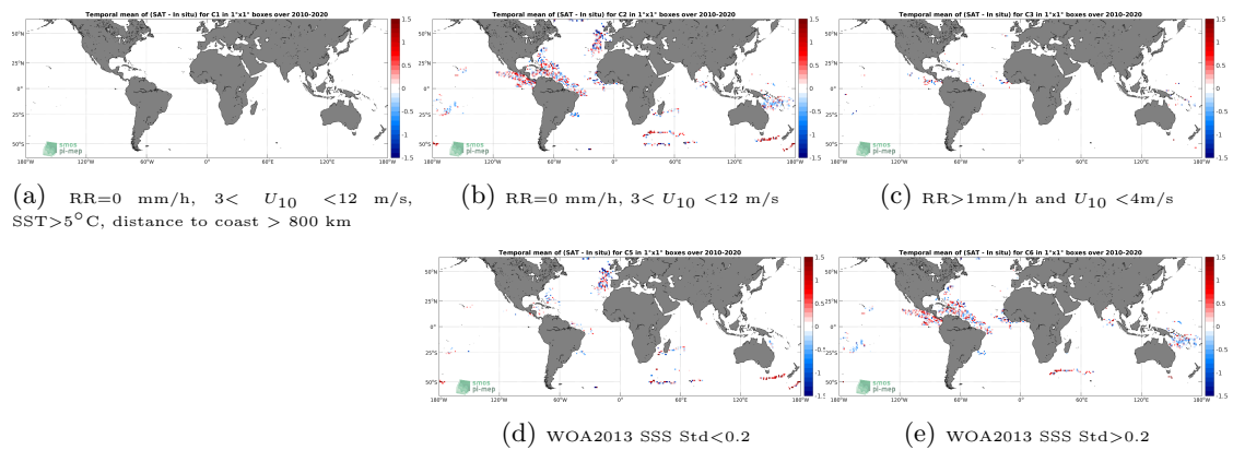
Figure 11: Temporal mean gridded over spatial boxes of size 1^\circ \times 1^\circ of \Delta\text{SSS} (SMOS SSS L2 v700 (ESA) - Surface drifters) for 5 different subdatasets corresponding to:RR=0 mm/h, 3 < U_{10} < 12 m/s, SST >5^\circ\text{C} , distance to coast > 800 km (a), RR=0 mm/h, 3 < U_{10} < 12 m/s (b), RR >1 mm/h and U_{10} < 4 m/s (c), WOA2013 SSS Std <0.2 (d), WOA2013 SSS Std >0.2 (e).
