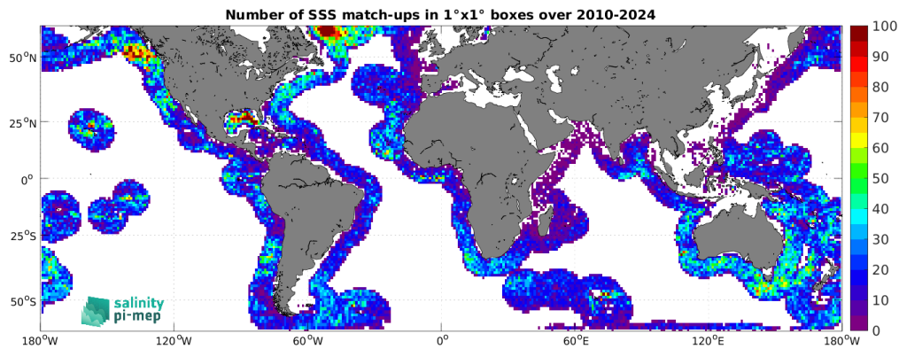
Figure 5: Number of SSS match-ups between Argo SSS and the SMOS SSS L2 v700 (ESA) SSS product for the SMOS coastal zone (<800km) 60N-60S Pi-MEP region over 1^\circ \times 1^\circ boxes and for the full satellite product period.
