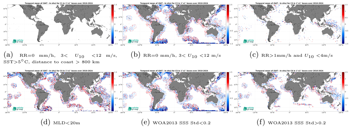
Figure 14: Temporal mean gridded over spatial boxes of size 1^\circ \times 1^\circ of \Delta SSS (SMOS SSS L2 v700 (ESA) - Argo) for 6 different subdatasets corresponding to:RR=0 mm/h, 3 < U_{10} < 12 m/s, SST > 5^\circ\text{C} , distance to coast > 800 km (a), RR=0 mm/h, 3 < U_{10} < 12 m/s (b), RR > 1 mm/h and U_{10} < 4 m/s (c),MLD < 20 m (d),WOA2013 SSS Std < 0.2 (e),WOA2013 SSS Std > 0.2 (f).
