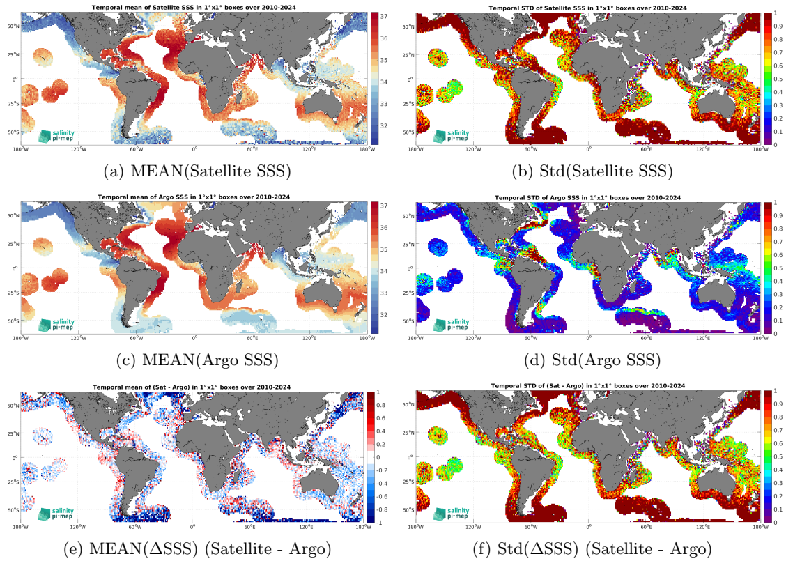
Figure 7: Temporal mean (left) and Std (right) of SSS from SMOS SSS L2 v700 (ESA) (top), Argo (middle), and of \Delta SSS (Satellite - Argo). Only match-up pairs are used to generate these maps.
