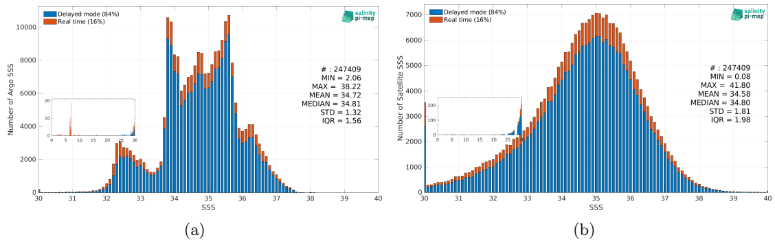
Figure 3: Histograms of SSS from Argo (a) and SMOS SSS L2 v700 (ESA) (b) considering all match-up pairs per bins of 0.1 over the SMOS coastal zone (<800km) 60N-60S Pi-MEP region and for the full satellite product period.
