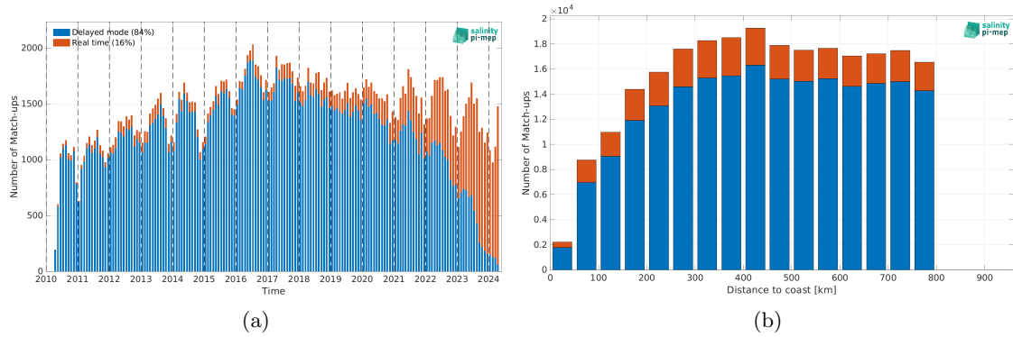
Figure 2: Number of match-ups between Argo and SMOS SSS L2 v700 (ESA) SSS as a function of time (a) and as function of the distance to coast (b) over the SMOS coastal zone (<800km) 60N-60S Pi-MEP region and for the full satellite product period.
