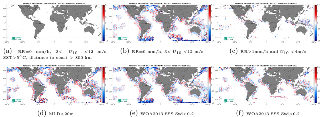
Figure 12: Temporal mean gridded over spatial boxes of size 1^\circ \times 1^\circ of \Delta SSS (SMOS SSS L2 v700 (ESA) - Argo) for 6 different subdatasets corresponding to: RR=0 mm/h, 3 < U_{10} < 12 m/s, SST > 5^\circ\text{C} , distance to coast > 800 km (a), RR=0 mm/h, 3 < U_{10} < 12 m/s (b), RR > 1 mm/h and U_{10} < 4 m/s (c),MLD < 20 m (d),WOA2013 SSS Std < 0.2 (e),WOA2013 SSS Std > 0.2 (f).
