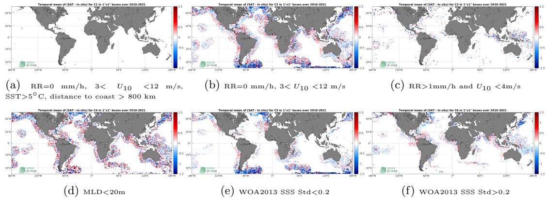
Figure 12: Temporal mean gridded over spatial boxes of size 1^\circ \times 1^\circ of \Delta SSS (SMOS SSS L2 v700 (ESA) - Argo) for 6 different subdatasets corresponding to:RR=0 mm/h, 3 < U_{10} < 12 m/s, SST > 5^\circ\text{C} , distance to coast > 800 km (a), RR=0 mm/h, 3 < U_{10} < 12 m/s (b), RR > 1 mm/h and U_{10} < 4 m/s (c),MLD < 20 m (d),WOA2013 SSS Std < 0.2 (e),WOA2013 SSS Std > 0.2 (f).
