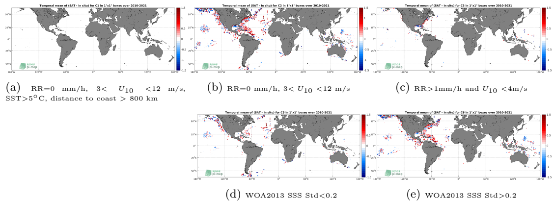
Figure 12: Temporal mean gridded over spatial boxes of size 1^\circ \times 1^\circ of \Delta SSS (SMOS SSS L2 v662 (ESA) - TSG (SAMOS)) for 5 different subdatasets corresponding to:RR=0 mm/h, 3 < U_{10} < 12 m/s, SST >5^\circ C, distance to coast > 800 km (a), RR=0 mm/h, 3 < U_{10} < 12 m/s (b), RR >1 mm/h and U_{10} < 4 m/s (c), WOA2013 SSS Std <0.2 (d), WOA2013 SSS Std >0.2 (e).
