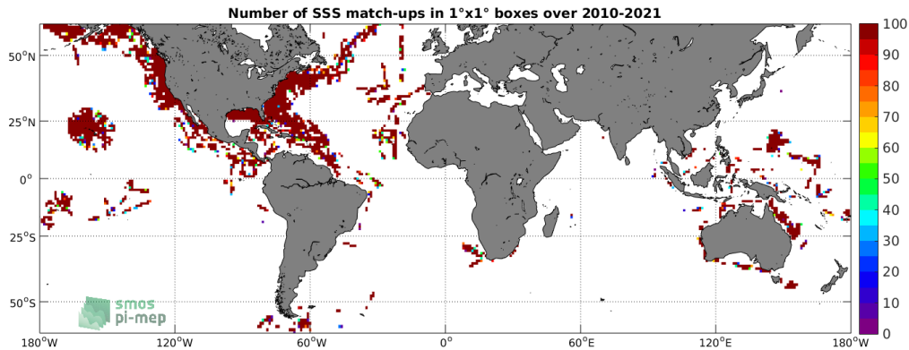
Figure 4: Number of SSS match-ups between TSG (SAMOS) SSS and the SMOS SSS L2 v662 (ESA) SSS product for the SMOS coastal zone (<800km) 60N-60S Pi-MEP region over 1^\circ \times 1^\circ boxes and for the full satellite product period.
