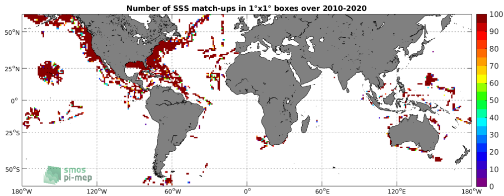
Figure 4: Number of SSS match-ups between TSG (SAMOS) SSS and the SMOS SSS L2 v662 (ESA) SSS product for the SMOS coastal zone (<800km) 60N-60S Pi-MEP region over 1°x1° boxes and for the full satellite product period.
