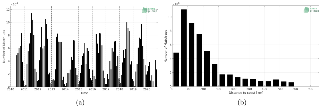
Figure 1: Number of match-ups between TSG (SAMOS) and SMOS SSS L2 v662 (ESA) SSS as a function of time (a) and as function of the distance to coast (b) over the SMOS coastal zone (<800km) 60N-60S Pi-MEP region and for the full satellite product period.
