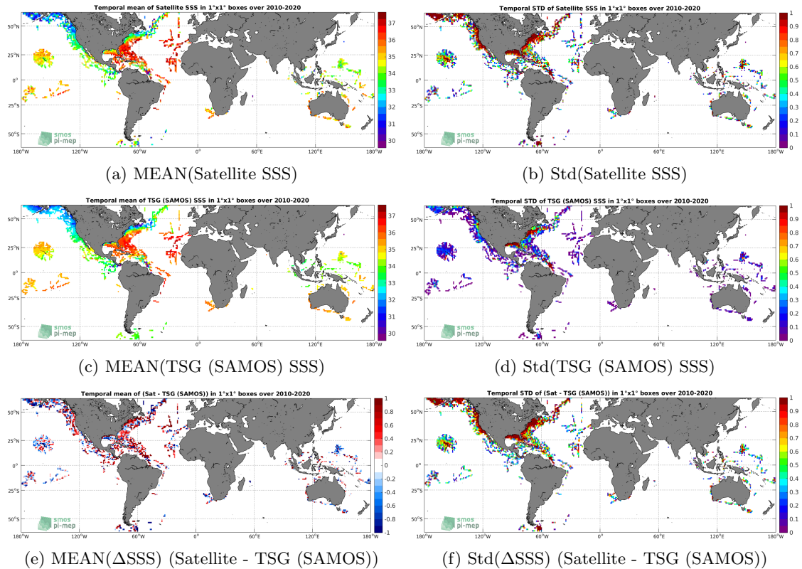
Figure 6: Temporal mean (left) and Std (right) of SSS from SMOS SSS L2 v662 (ESA) (top), TSG (SAMOS) (middle), and of \Delta SSS (Satellite - TSG (SAMOS)). Only match-up pairs are used to generate these maps.
