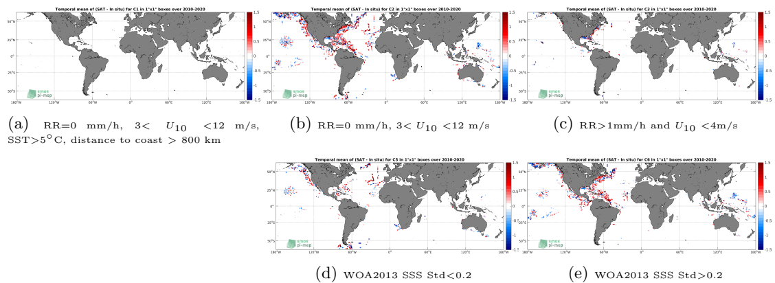
Figure 12: Temporal mean gridded over spatial boxes of size 1°x1° of \Delta SSS (SMOS SSS L2 v662 (ESA) - TSG (SAMOS)) for 5 different subdatasets corresponding to:RR=0 mm/h, 3 < U_{10} < 12 m/s, SST > 5°C, distance to coast > 800 km (a), RR=0 mm/h, 3 < U_{10} < 12 m/s (b), RR > 1mm/h and U_{10} < 4 m/s (c), WOA2013 SSS Std < 0.2 (d), WOA2013 SSS Std > 0.2 (e).
