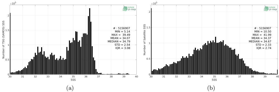
Figure 2: Histograms of SSS from TSG (SAMOS) (a) and SMOS SSS L2 v662 (ESA) (b) considering all match-up pairs per bins of 0.1 over the SMOS coastal zone (<800km) 60N-60S Pi-MEP region and for the full satellite product period.
