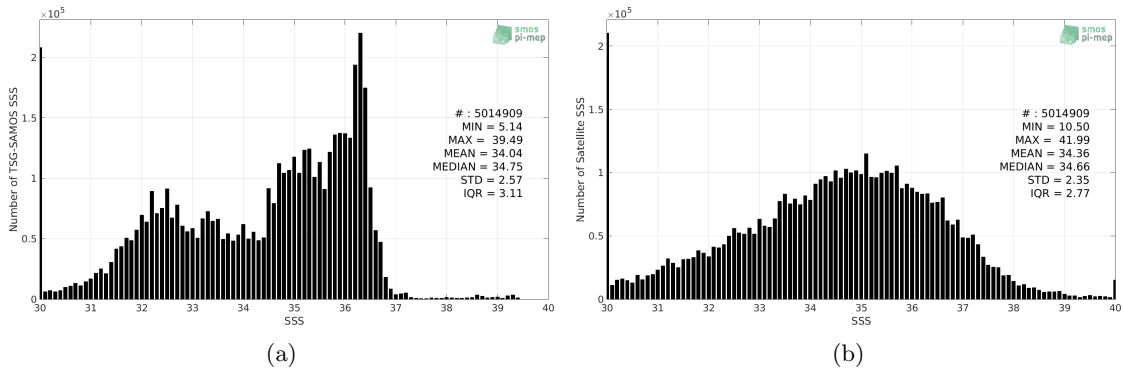
Figure 2: Histograms of SSS from TSG-SAMOS (a) and SMOS L2 v662 (ESA) (b) considering all match-up pairs per bins of 0.1 over the SMOS coastal zone (<800km) 60N-60S Pi-MEP region and for the full satellite product period.
