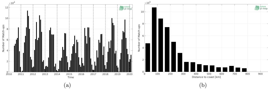
Figure 1: Number of match-ups between TSG-SAMOS and SMOS L2 v662 (ESA) SSS as a function of time (a) and as function of the distance to coast (b) over the SMOS coastal zone (<800km) 60N-60S Pi-MEP region and for the full satellite product period.
