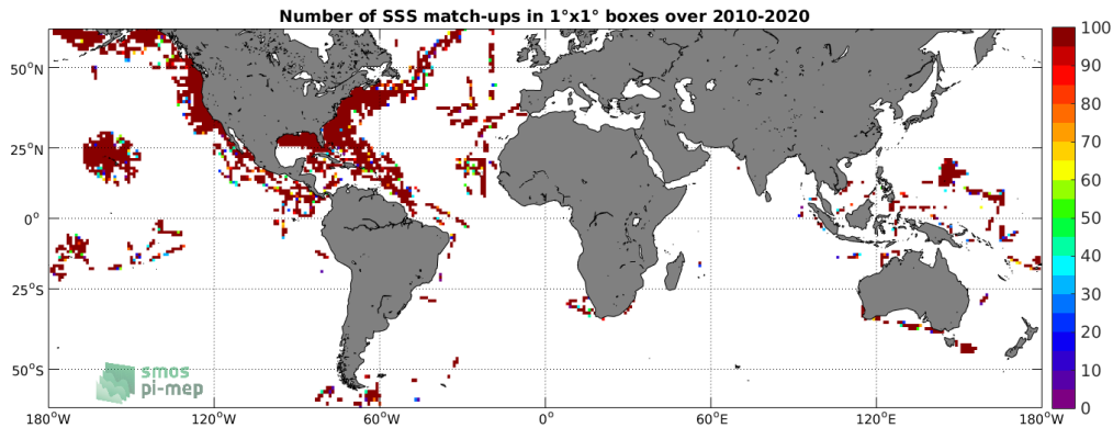
Figure 4: Number of SSS match-ups between TSG-SAMOS SSS and the SMOS L2 v662 (ESA) SSS product for the SMOS coastal zone (<800km) 60N-60S Pi-MEP region over 1^\circ \times 1^\circ boxes and for the full satellite product period.
