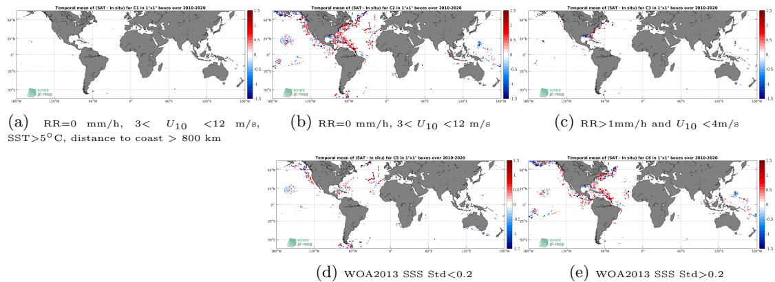
Figure 12: Temporal mean gridded over spatial boxes of size 1^\circ \times 1^\circ of \Delta SSS (SMOS L2 v662 (ESA) - TSG-SAMOS) for 5 different subdatasets corresponding to:RR=0 mm/h, 3 < U_{10} < 12 m/s, SST >5^\circ\text{C} , distance to coast > 800 km (a), RR=0 mm/h, 3 < U_{10} < 12 m/s (b), RR >1 mm/h and U_{10} < 4 m/s (c), WOA2013 SSS Std <0.2 (d), WOA2013 SSS Std >0.2 (e).
