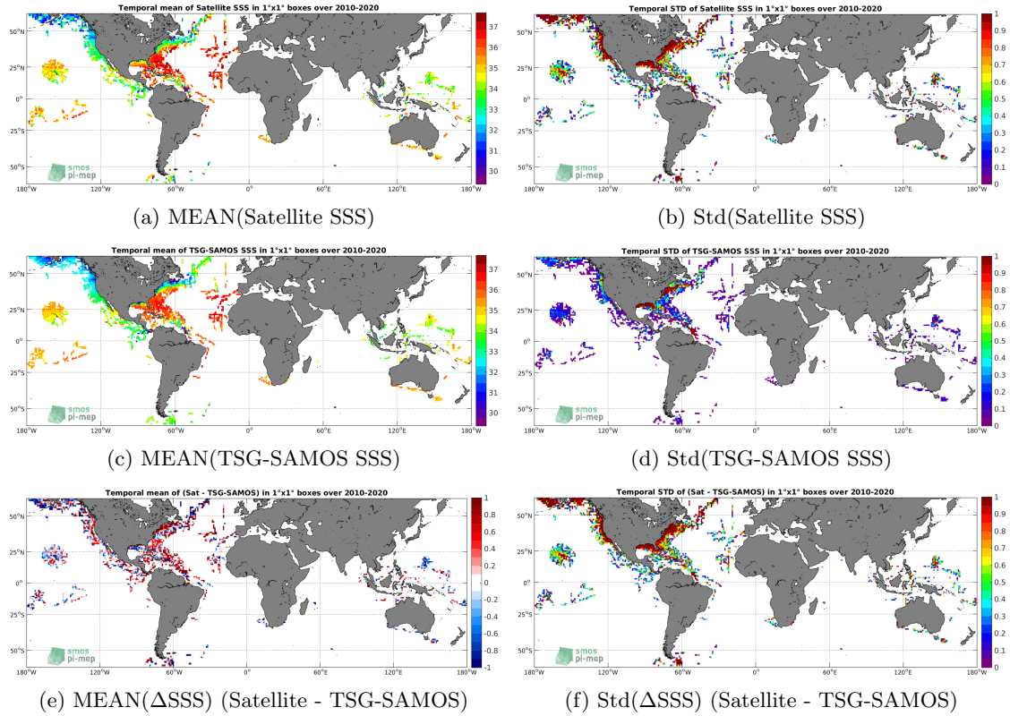
Figure 6: Temporal mean (left) and Std (right) of SSS from SMOS L2 v662 (ESA) (top), TSG-SAMOS (middle), and of \Delta SSS (Satellite - TSG-SAMOS). Only match-up pairs are used to generate these maps.
