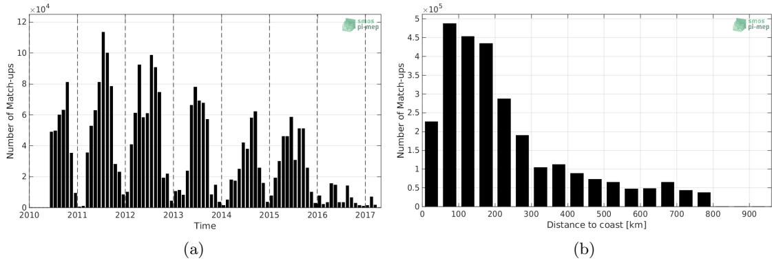
Figure 1: Number of match-ups between TSG-SAMOS and SMOS-L2-DPGS-v662 SSS as a function of time (a) and as function of the distance to coast (b) over the SMOS coastal zone ( \leq 800 km) 60N-60S Pi-MEP region and for the full satellite product period.
