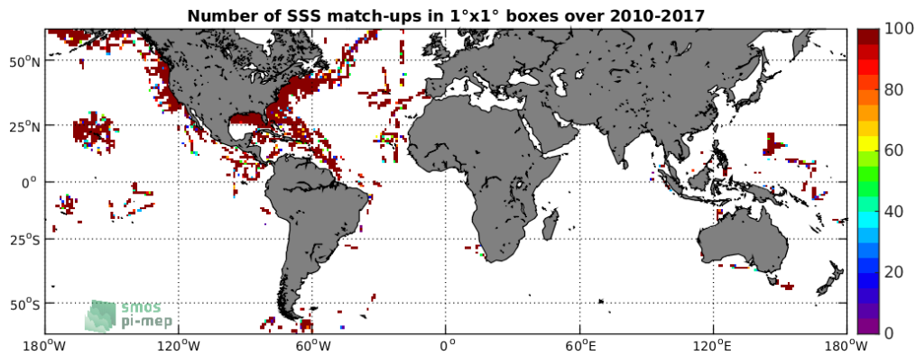
Figure 4: Number of SSS match-ups between TSG-SAMOS SSS and the SMOS-L2-DPGS-v662 SSS product for the SMOS coastal zone ( \geq 800\text{km} ) 60N-60S Pi-MEP region over 1^\circ \times 1^\circ boxes and for the full satellite product period.
