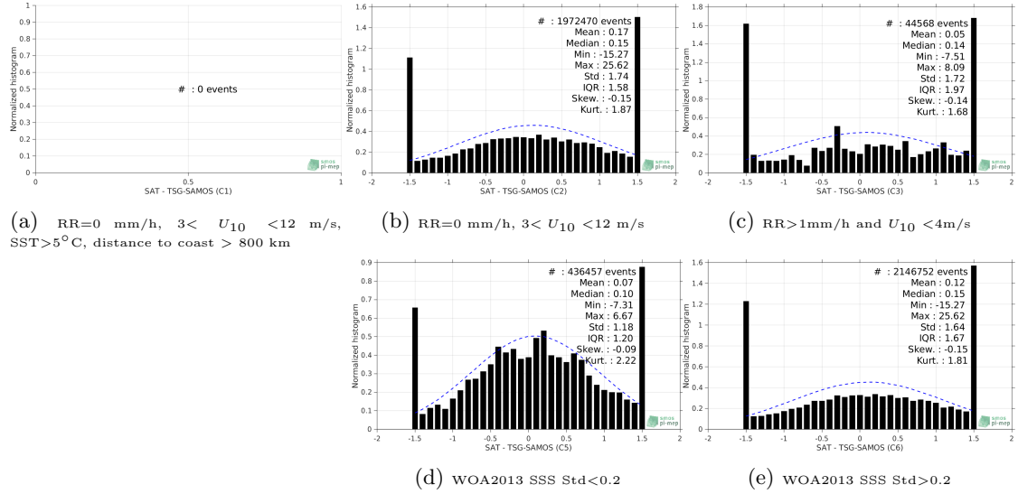
Figure 13: Normalized histogram of \Delta\text{SSS} (SMOS-L2-DPGS-v662 - TSG-SAMOS) for 5 different subdatasets corresponding to: RR=0 mm/h, 3 < U_{10} < 12 m/s, SST >5^{\circ}\text{C} , distance to coast > 800 km (a), RR=0 mm/h, 3 < U_{10} < 12 m/s (b), RR>1\text{mm/h} and U_{10} < 4\text{m/s} (c), WOA2013 SSS Std <0.2 (d), WOA2013 SSS Std >0.2 (e).
