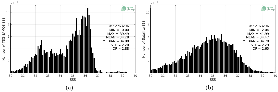
Figure 2: Histograms of SSS from TSG-SAMOS (a) and SMOS-L2-DPGS-v662 (b) considering all match-up pairs per bins of 0.1 over the SMOS coastal zone ( \leq 800 km) 60N-60S Pi-MEP region and for the full satellite product period.
