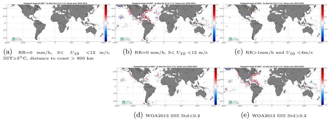
Figure 12: Temporal mean gridded over spatial boxes of size 1^\circ \times 1^\circ of \Delta SSS (SMOS-L2-DPGS-v662 - TSG-SAMOS) for 5 different subdatasets corresponding to:RR=0 mm/h, 3 < U_{10} < 12 m/s, SST >5^\circ C, distance to coast > 800 km (a), RR=0 mm/h, 3 < U_{10} < 12 m/s (b), RR >1 mm/h and U_{10} < 4 m/s (c), WOA2013 SSS Std <0.2 (d), WOA2013 SSS Std >0.2 (e).
