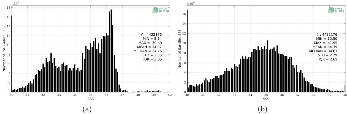
Figure 2: Histograms of SSS from TSG-SAMOS (a) and SMOS-L2-DPGS-v662 (b) considering all match-up pairs per bins of 0.1 over the SMOS coastal zone ( \pm 800\text{km} ) 60N-60S Pi-MEP region and for the full satellite product period.
