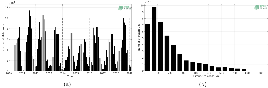
Figure 1: Number of match-ups between TSG-SAMOS and SMOS-L2-DPGS-v662 SSS as a function of time (a) and as function of the distance to coast (b) over the SMOS coastal zone ( \pm 800\text{km} ) 60N-60S Pi-MEP region and for the full satellite product period.
