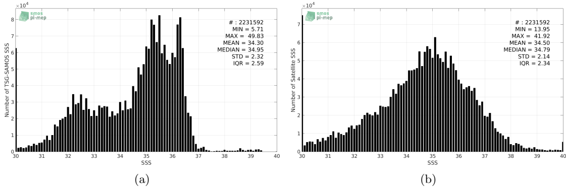
Figure 2: Histograms of SSS from TSG-SAMOS (a) and SMOS-L2-DPGS-v662 (b) considering all match-up pairs per bins of 0.1 over the SMOS coastal zone ( \approx 800 km) 60N-60S Pi-MEP region and for the full satellite product period.
