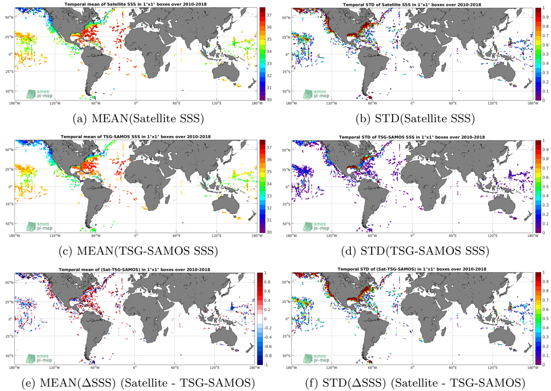
Figure 6: Temporal mean (left) and STD (right) of SSS from SMOS-L2-DPGS-v662 (top), TSG-SAMOS (middle), and of \Delta SSS (Satellite - TSG-SAMOS). Only match-up pairs are used to generate these maps.
