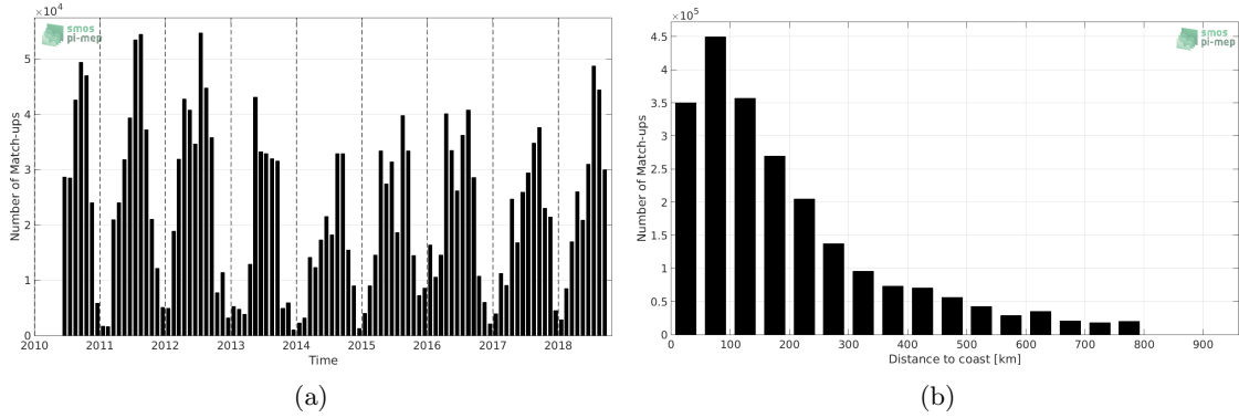
Figure 1: Number of match-ups between TSG-SAMOS and SMOS-L2-DPGS-v662 SSS as a function of time (a) and as function of the distance to coast (b) over the SMOS coastal zone ( \approx 800 km) 60N-60S Pi-MEP region and for the full satellite product period.
