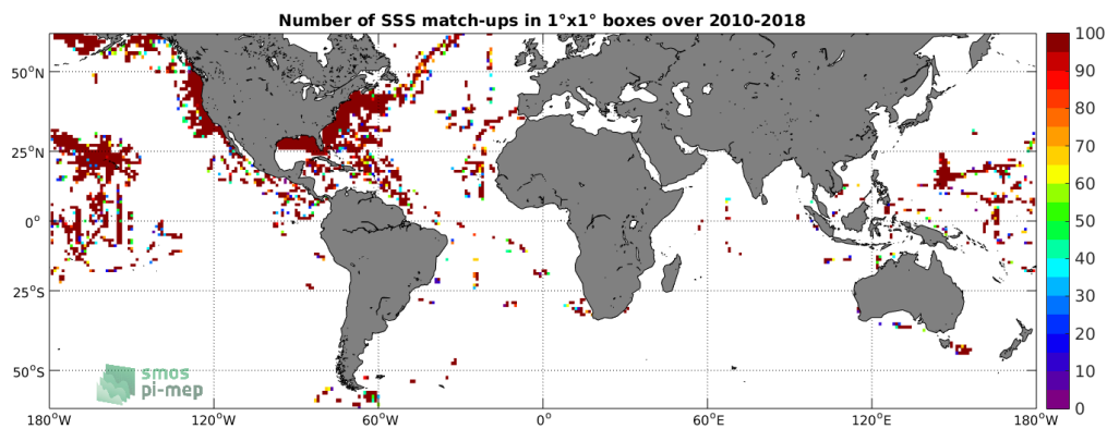
Figure 4: Number of SSS match-ups between TSG-SAMOS SSS and the SMOS-L2-DPGS-v662 SSS product for the SMOS coastal zone ( \pm 800\text{km} ) 60N-60S Pi-MEP region over 1^\circ \times 1^\circ boxes and for the full satellite product period.
