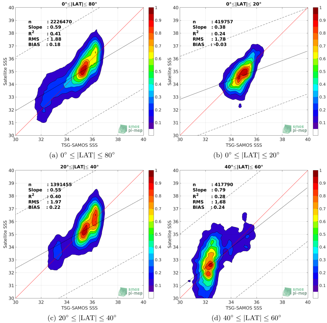
Figure 9: Contour maps of the concentration of SMOS-L2-DPGS-v662 SSS (y-axis) versus TSG-SAMOS SSS (x-axis) at match-up pairs for different latitude bands. For each plot, the red line shows x=y . The black thin and dashed lines indicate a linear fit through the data cloud and the \pm 95\% confidence levels, respectively. The number match-up pairs n , the slope and R^2 coefficient of the linear fit, the root mean square (RMS) and the mean bias between satellite and in situ data are indicated for each latitude band in each plots.
