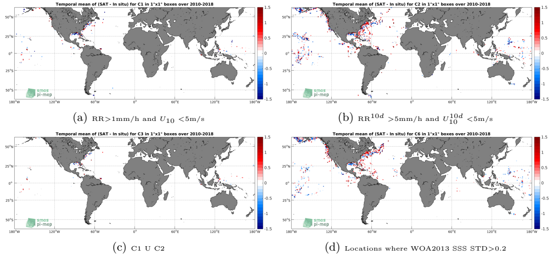
Figure 12: Temporal mean gridded over spatial boxes of size 1^\circ \times 1^\circ of \Delta SSS (SMOS-L2-DPGS-v662 - TSG-SAMOS) for 4 different subdatasets corresponding to: RR > 1\text{mm/h} and U_{10} < 5\text{m/s} (a), RR^{10d} > 5\text{mm/h} and U_{10}^{10d} < 5\text{m/s} (b), C1 U C2 (c), Locations where WOA2013 SSS STD > 0.2 (d).
