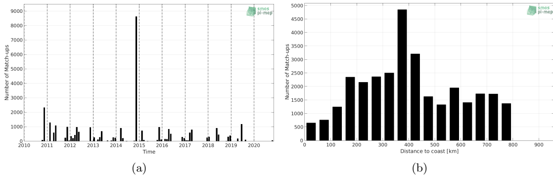
Figure 1: Number of match-ups between TSG (Polarstern) and SMOS SSS L2 v662 (ESA) SSS as a function of time (a) and as function of the distance to coast (b) over the SMOS coastal zone (<800km) 60N-60S Pi-MEP region and for the full satellite product period.
