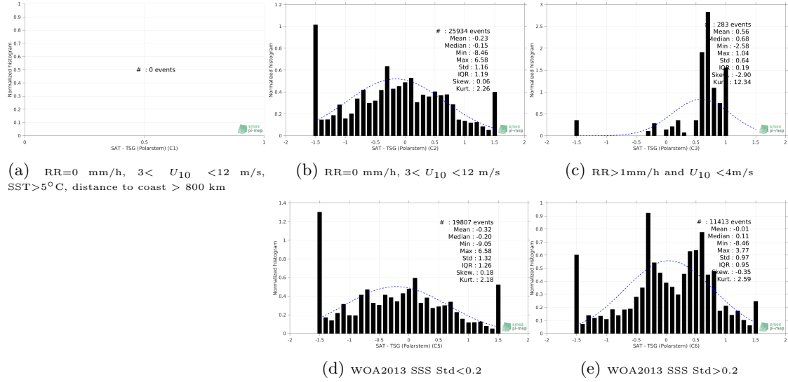
Figure 13: Normalized histogram of \Delta SSS (SMOS SSS L2 v662 (ESA) - TSG (Polarstern)) for 5 different subdatasets corresponding to: RR=0 mm/h, 3 < U_{10} < 12 m/s, SST > 5°C, distance to coast > 800 km (a), RR=0 mm/h, 3 < U_{10} < 12 m/s (b), RR > 1mm/h and U_{10} < 4 m/s (c), WOA2013 SSS Std < 0.2 (d), WOA2013 SSS Std > 0.2 (e).
