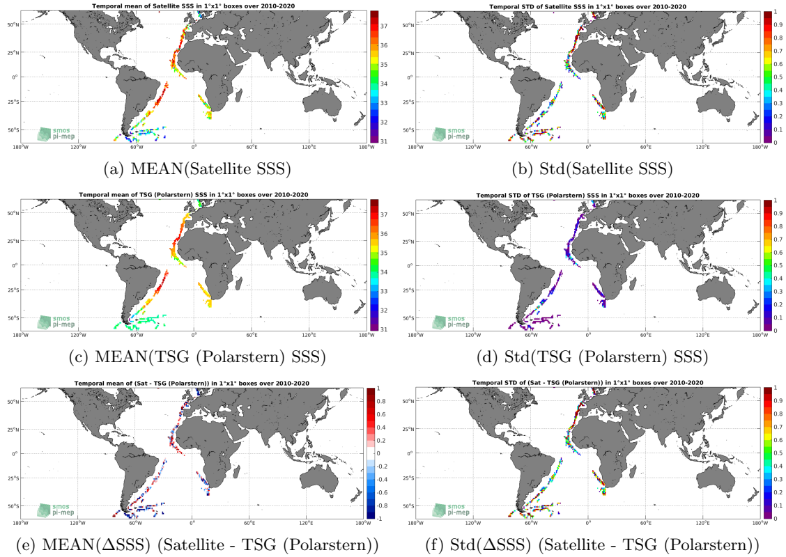
Figure 6: Temporal mean (left) and Std (right) of SSS from SMOS SSS L2 v662 (ESA) (top), TSG (Polarstern) (middle), and of \Delta SSS (Satellite - TSG (Polarstern)). Only match-up pairs are used to generate these maps.
