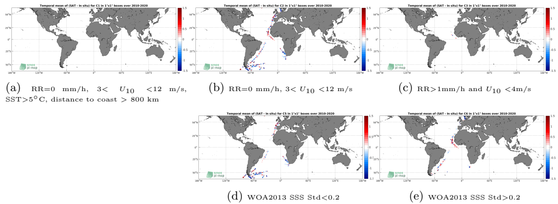
Figure 12: Temporal mean gridded over spatial boxes of size 1^\circ \times 1^\circ of \Delta SSS (SMOS SSS L2 v662 (ESA) - TSG (Polarstern)) for 5 different subdatasets corresponding to:RR=0 mm/h, 3 < U_{10} < 12 m/s, SST >5^\circ C, distance to coast > 800 km (a), RR=0 mm/h, 3 < U_{10} < 12 m/s (b), RR >1 mm/h and U_{10} < 4 m/s (c), WOA2013 SSS Std <0.2 (d), WOA2013 SSS Std >0.2 (e).
