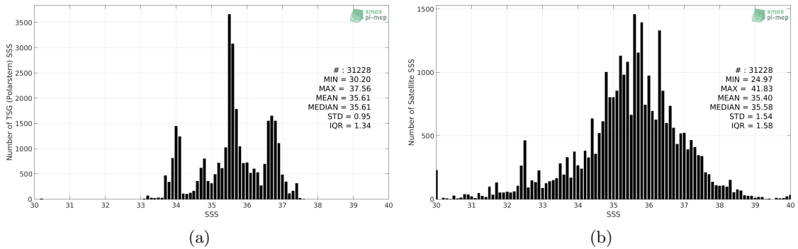
Figure 2: Histograms of SSS from TSG (Polarstern) (a) and SMOS SSS L2 v662 (ESA) (b) considering all match-up pairs per bins of 0.1 over the SMOS coastal zone (<800km) 60N-60S Pi-MEP region and for the full satellite product period.
