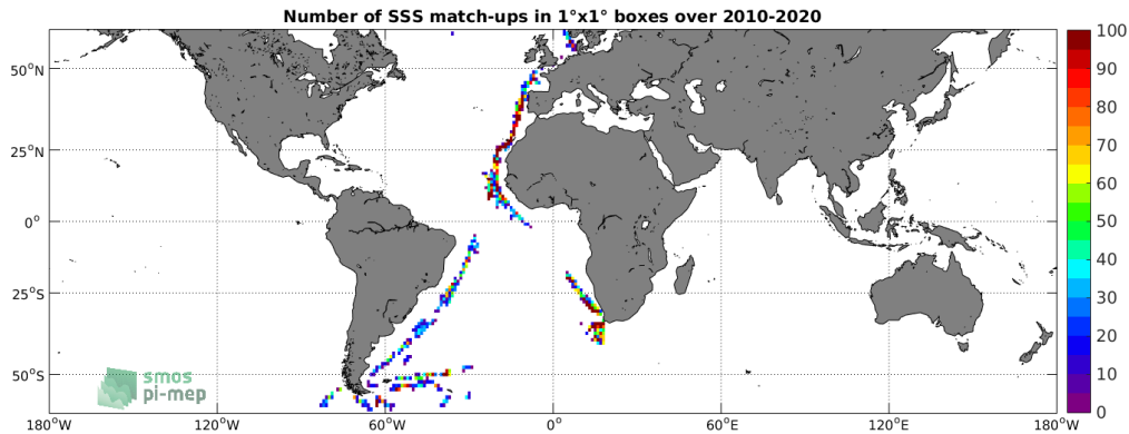
Figure 4: Number of SSS match-ups between TSG (Polarstern) SSS and the SMOS SSS L2 v662 (ESA) SSS product for the SMOS coastal zone (<800km) 60N-60S Pi-MEP region over 1°x1° boxes and for the full satellite product period.
