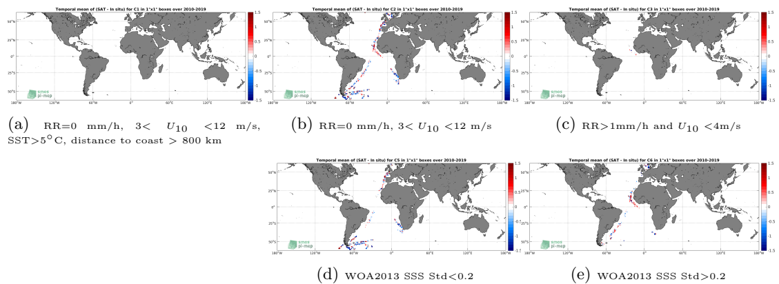
Figure 12: Temporal mean gridded over spatial boxes of size 1°x1° of \Delta SSS (SMOS SSS L2 v662 (ESA) - TSG (Polarstern)) for 5 different subdatasets corresponding to: RR=0 mm/h, 3 < U_{10} < 12 m/s, SST > 5°C, distance to coast > 800 km (a), RR=0 mm/h, 3 < U_{10} < 12 m/s (b), RR > 1mm/h and U_{10} < 4 m/s (c), WOA2013 SSS Std < 0.2 (d), WOA2013 SSS Std > 0.2 (e).
