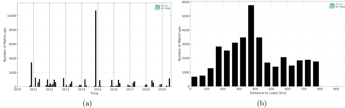
Figure 1: Number of match-ups between TSG-POLARSTERN and SMOS L2 v662 (ESA) SSS as a function of time (a) and as function of the distance to coast (b) over the SMOS coastal zone (<800km) 60N-60S Pi-MEP region and for the full satellite product period.
