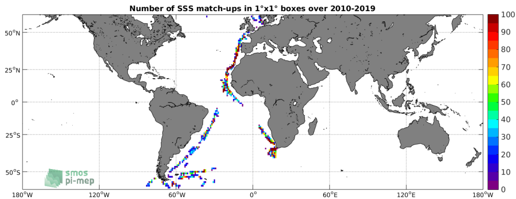
Figure 4: Number of SSS match-ups between TSG-POLARSTERN SSS and the SMOS L2 v662 (ESA) SSS product for the SMOS coastal zone (<800km) 60N-60S Pi-MEP region over 1^\circ \times 1^\circ boxes and for the full satellite product period.
