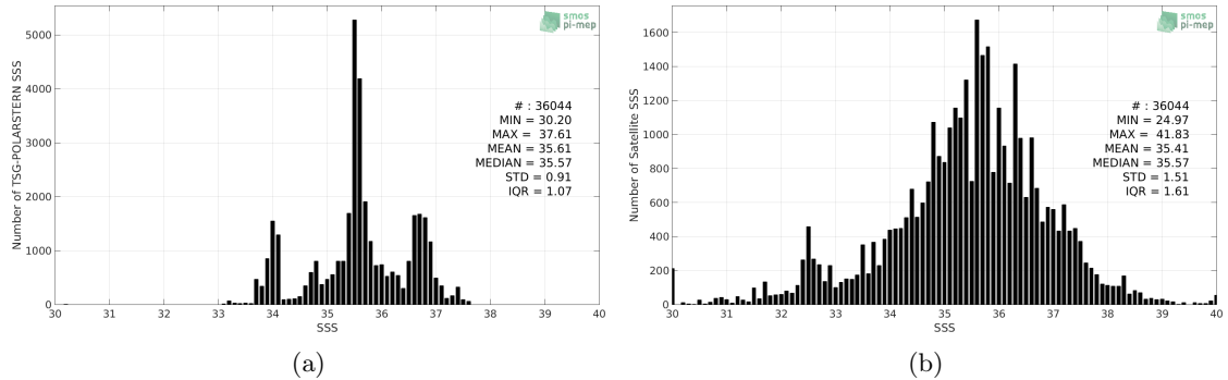
Figure 2: Histograms of SSS from TSG-POLARSTERN (a) and SMOS L2 v662 (ESA) (b) considering all match-up pairs per bins of 0.1 over the SMOS coastal zone (<800km) 60N-60S Pi-MEP region and for the full satellite product period.
