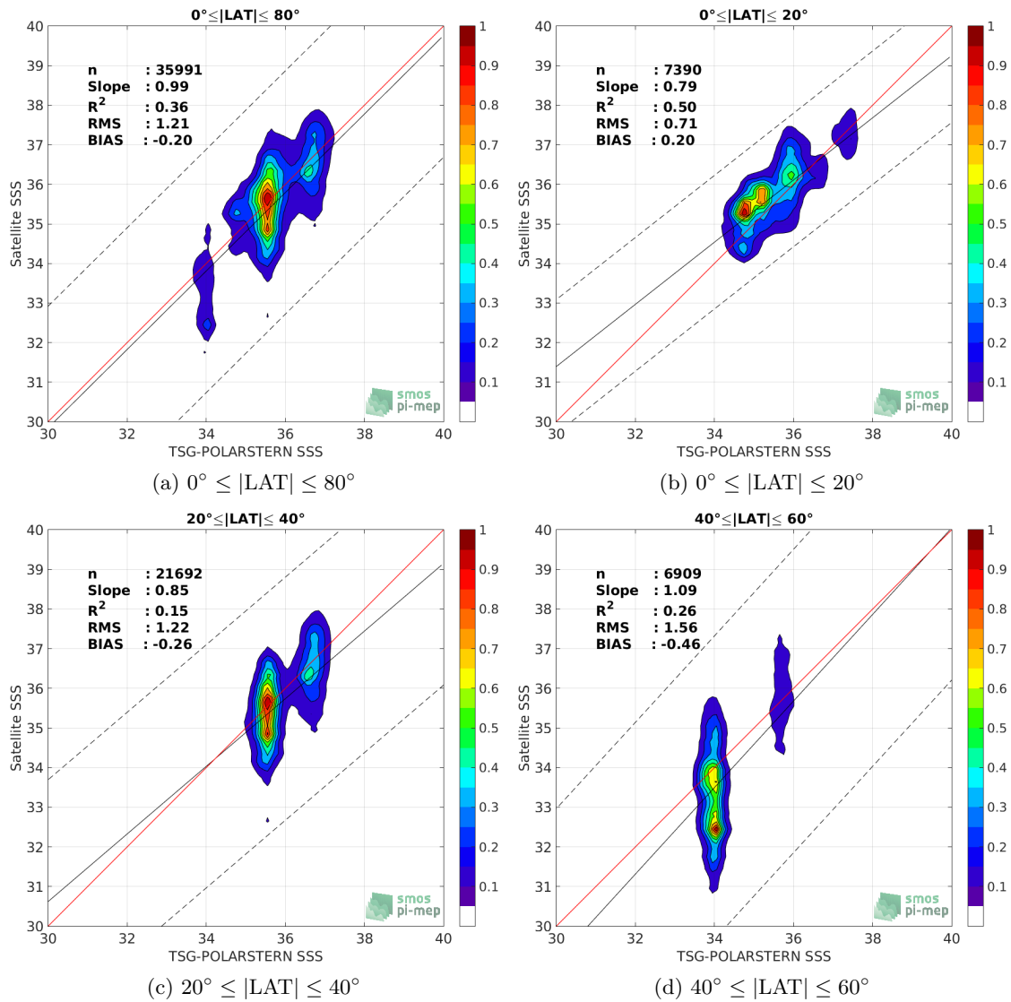
Figure 9: Contour maps of the concentration of SMOS L2 v662 (ESA) SSS ( y -axis) versus TSG-POLARSTERN SSS ( x -axis) at match-up pairs for different latitude bands. For each plot, the red line shows x=y . The black thin and dashed lines indicate a linear fit through the data cloud and the \pm 95\% confidence levels, respectively. The number match-up pairs n , the slope and R^2 coefficient of the linear fit, the root mean square (RMS) and the mean bias between satellite and in situ data are indicated for each latitude band in each plots.
