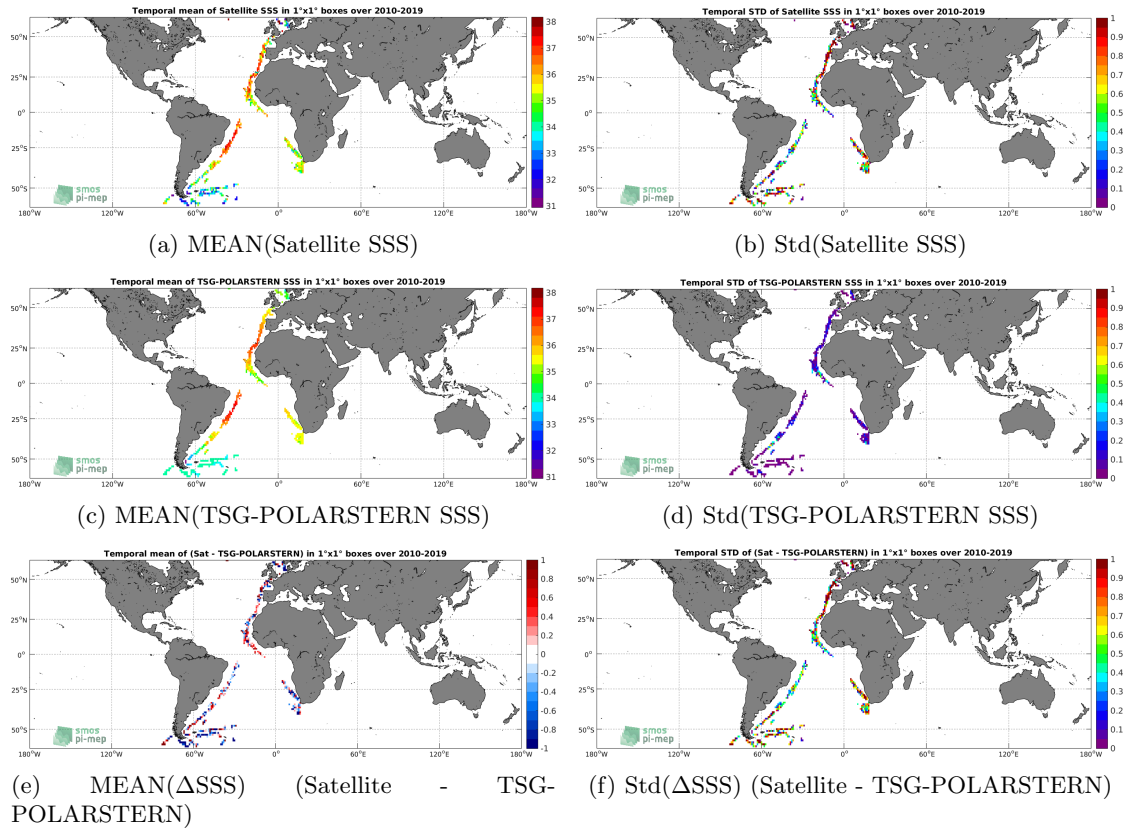
Figure 6: Temporal mean (left) and Std (right) of SSS from SMOS L2 v662 (ESA) (top), TSG-POLARSTERN (middle), and of \Delta SSS (Satellite - TSG-POLARSTERN). Only match-up pairs are used to generate these maps.
