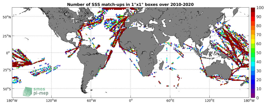
Figure 4: Number of SSS match-ups between TSG (LEGOS-DM) SSS and the SMOS SSS L2 v662 (ESA) SSS product for the SMOS coastal zone ( <800\text{km} ) 60\text{N} - 60\text{S} Pi-MEP region over 1^\circ \times 1^\circ boxes and for the full satellite product period.
