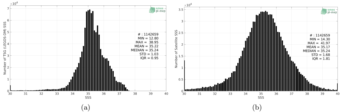
Figure 2: Histograms of SSS from TSG (LEGOS-DM) (a) and SMOS SSS L2 v662 (ESA) (b) considering all match-up pairs per bins of 0.1 over the SMOS coastal zone (<800km) 60N-60S Pi-MEP region and for the full satellite product period.
