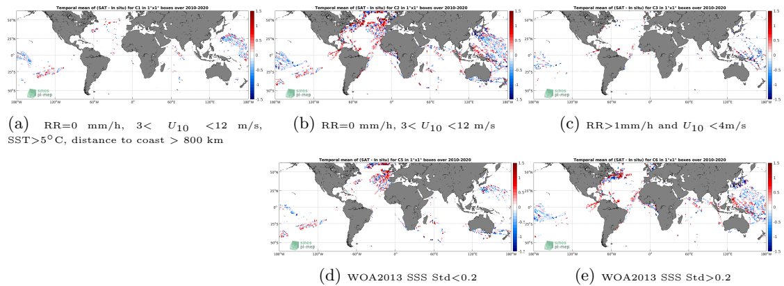
Figure 12: Temporal mean gridded over spatial boxes of size 1^\circ \times 1^\circ of \Delta SSS (SMOS SSS L2 v662 (ESA) - TSG (LEGOS-DM)) for 5 different subdatasets corresponding to:RR=0 mm/h, 3 < U_{10} < 12 m/s, SST >5^\circ\text{C} , distance to coast > 800 km (a), RR=0 mm/h, 3 < U_{10} < 12 m/s (b), RR >1 mm/h and U_{10} < 4 m/s (c), WOA2013 SSS Std <0.2 (d), WOA2013 SSS Std >0.2 (e).
