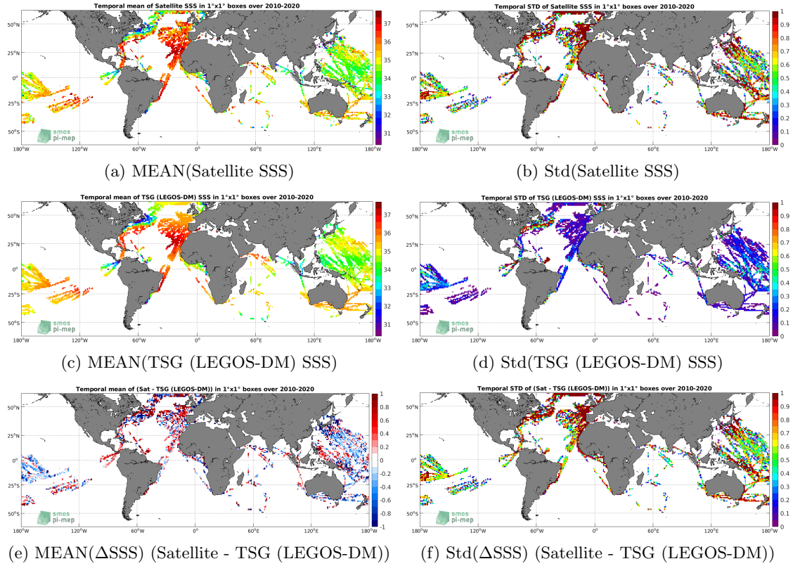
Figure 6: Temporal mean (left) and Std (right) of SSS from SMOS SSS L2 v662 (ESA) (top), TSG (LEGOS-DM) (middle), and of \Delta SSS (Satellite - TSG (LEGOS-DM)). Only match-up pairs are used to generate these maps.
