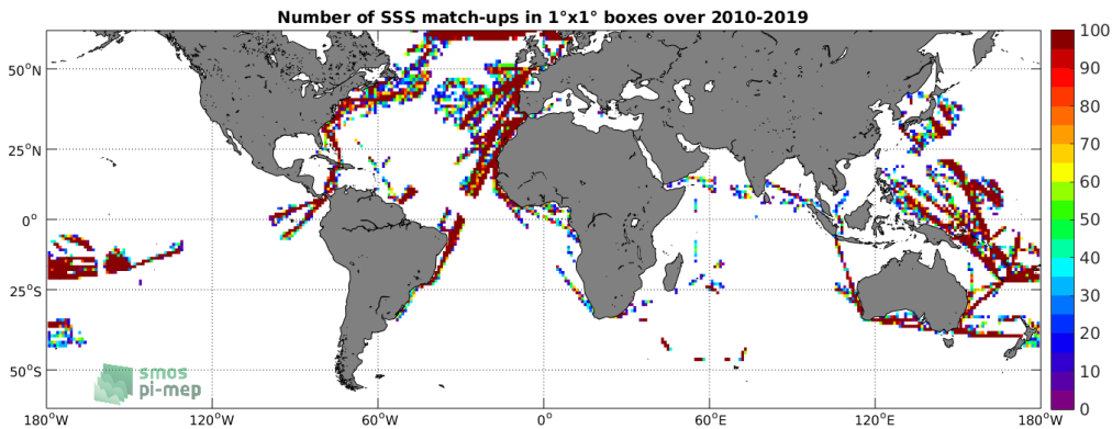
Figure 4: Number of SSS match-ups between TSG (LEGOS-DM) SSS and the SMOS SSS L2 v662 (ESA) SSS product for the SMOS coastal zone (<800km) 60N-60S Pi-MEP region over 1°x1° boxes and for the full satellite product period.
