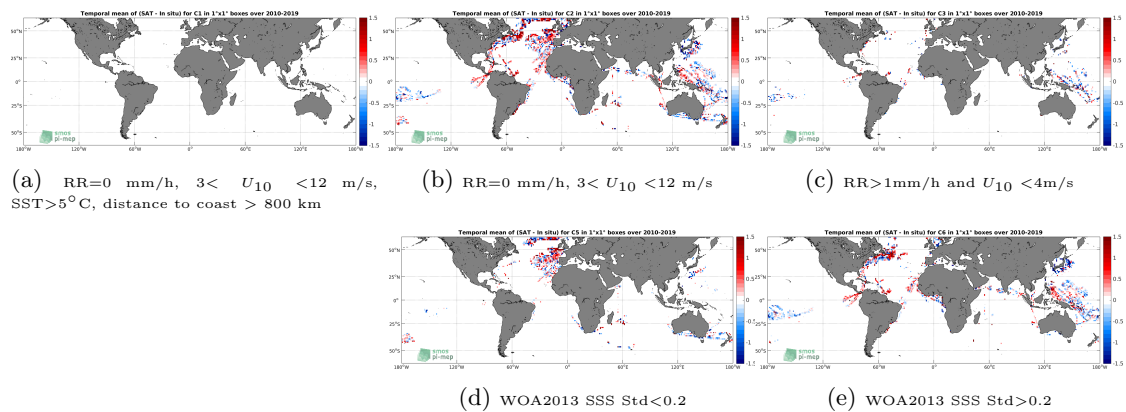
Figure 12: Temporal mean gridded over spatial boxes of size 1^\circ \times 1^\circ of \Delta SSS (SMOS SSS L2 v662 (ESA) - TSG (LEGOS-DM)) for 5 different subdatasets corresponding to: RR=0 mm/h, 3 < U_{10} < 12 m/s, SST > 5°C, distance to coast > 800 km (a), RR=0 mm/h, 3 < U_{10} < 12 m/s (b), RR > 1mm/h and U_{10} < 4 m/s (c), WOA2013 SSS Std < 0.2 (d), WOA2013 SSS Std > 0.2 (e).
