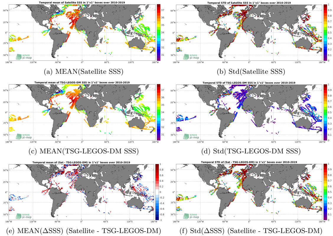
Figure 6: Temporal mean (left) and Std (right) of SSS from SMOS L2 v662 (ESA) (top), TSG-LEGOS-DM (middle), and of \Delta SSS (Satellite - TSG-LEGOS-DM). Only match-up pairs are used to generate these maps.
