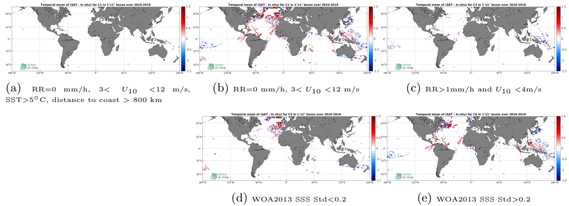
Figure 12: Temporal mean gridded over spatial boxes of size 1^\circ \times 1^\circ of \Delta SSS (SMOS L2 v662 (ESA) - TSG-LEGOS-DM) for 5 different subdatasets corresponding to:RR=0 mm/h, 3 < U_{10} < 12 m/s, SST >5^\circ C, distance to coast > 800 km (a), RR=0 mm/h, 3 < U_{10} < 12 m/s (b), RR >1 mm/h and U_{10} < 4 m/s (c), WOA2013 SSS Std <0.2 (d), WOA2013 SSS Std >0.2 (e).
