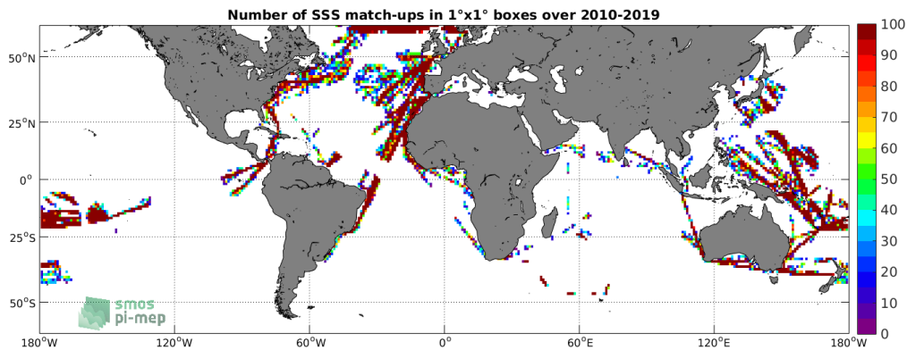
Figure 4: Number of SSS match-ups between TSG-LEGOS-DM SSS and the SMOS L2 v662 (ESA) SSS product for the SMOS coastal zone (<800km) 60N-60S Pi-MEP region over 1^\circ \times 1^\circ boxes and for the full satellite product period.
