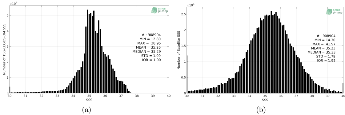
Figure 2: Histograms of SSS from TSG-LEGOS-DM (a) and SMOS L2 v662 (ESA) (b) considering all match-up pairs per bins of 0.1 over the SMOS coastal zone (<800km) 60N-60S Pi-MEP region and for the full satellite product period.
