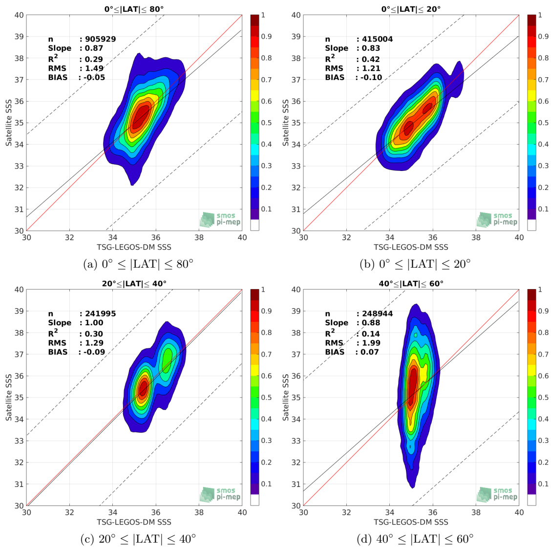
Figure 9: Contour maps of the concentration of SMOS L2 v662 (ESA) SSS ( y -axis) versus TSG-LEGOS-DM SSS ( x -axis) at match-up pairs for different latitude bands. For each plot, the red line shows x=y . The black thin and dashed lines indicate a linear fit through the data cloud and the \pm 95\% confidence levels, respectively. The number match-up pairs n , the slope and R^2 coefficient of the linear fit, the root mean square (RMS) and the mean bias between satellite and in situ data are indicated for each latitude band in each plots.
