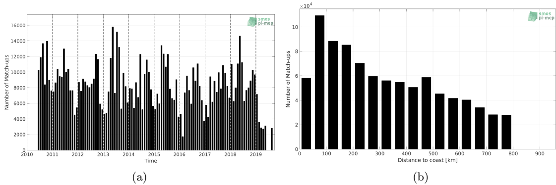
Figure 1: Number of match-ups between TSG-LEGOS-DM and SMOS L2 v662 (ESA) SSS as a function of time (a) and as function of the distance to coast (b) over the SMOS coastal zone (<800km) 60N-60S Pi-MEP region and for the full satellite product period.
