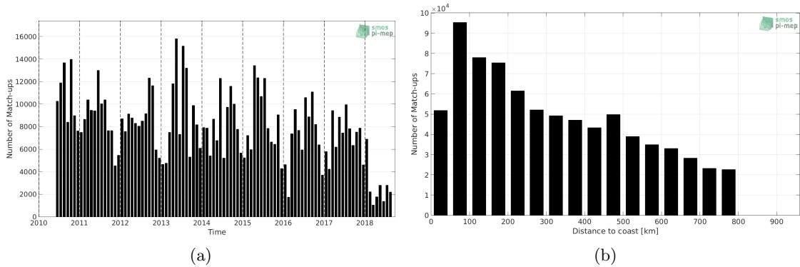
Figure 1: Number of match-ups between TSG-LEGOS-DM and SMOS-L2-DPGS-v662 SSS as a function of time (a) and as function of the distance to coast (b) over the SMOS coastal zone ( \pm 800 km) 60N-60S Pi-MEP region and for the full satellite product period.
