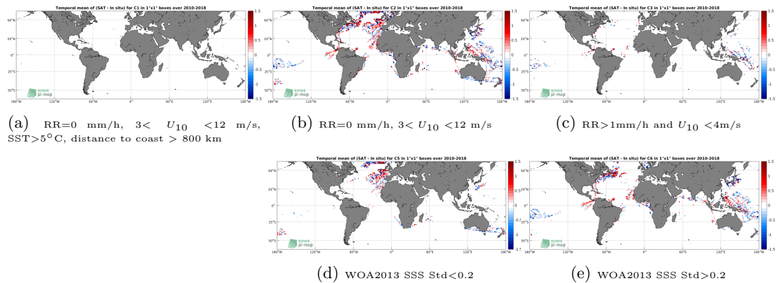
Figure 12: Temporal mean gridded over spatial boxes of size 1^\circ \times 1^\circ of \Delta SSS (SMOS-L2-DPGS-v662 - TSG-LEGOS-DM) for 5 different subdatasets corresponding to:RR=0 mm/h, 3 < U_{10} < 12 m/s, SST >5^\circ\text{C} , distance to coast > 800 km (a), RR=0 mm/h, 3 < U_{10} < 12 m/s (b), RR >1 mm/h and U_{10} < 4 m/s (c), WOA2013 SSS Std <0.2 (d), WOA2013 SSS Std >0.2 (e).
