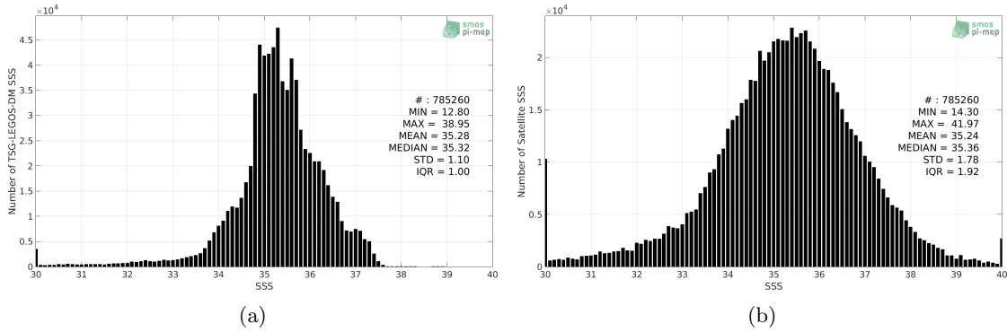
Figure 2: Histograms of SSS from TSG-LEGOS-DM (a) and SMOS-L2-DPGS-v662 (b) considering all match-up pairs per bins of 0.1 over the SMOS coastal zone ( \pm 800 km) 60N-60S Pi-MEP region and for the full satellite product period.
