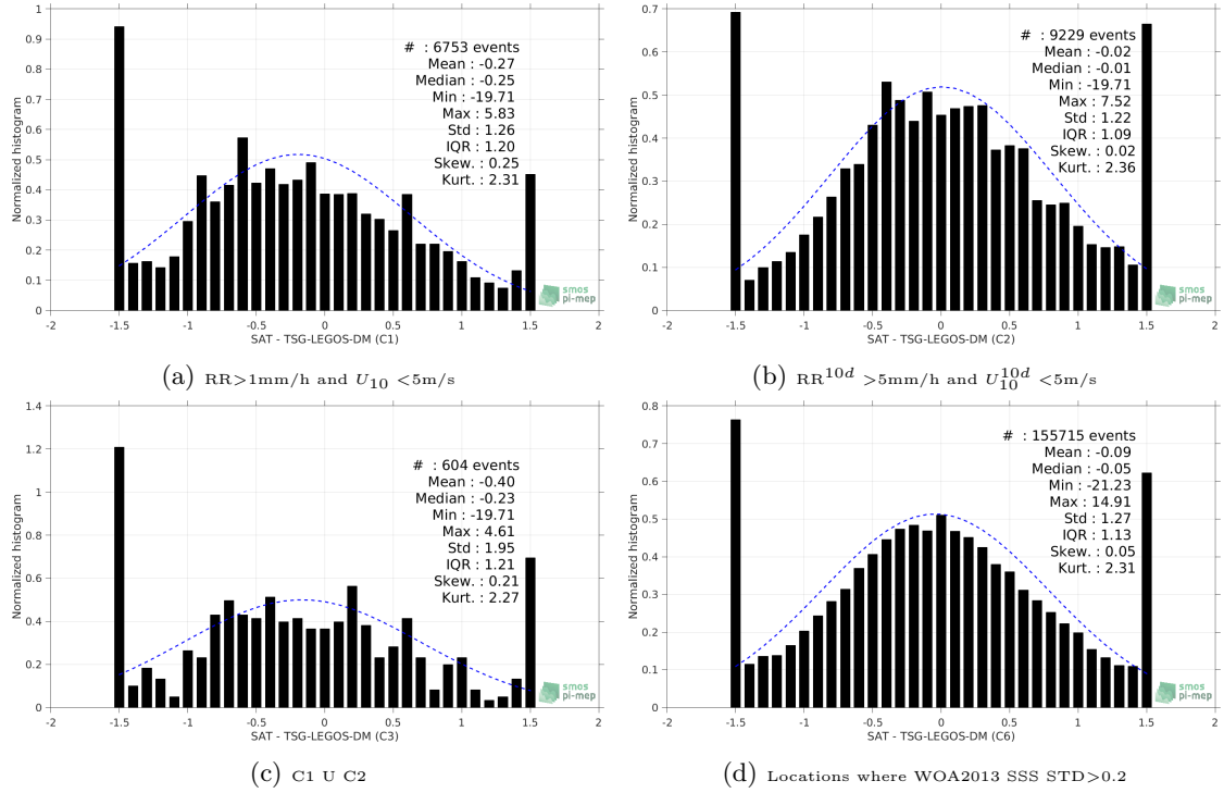
Figure 13: Normalized histogram of \Delta SSS (SMOS-L2-DPGS-v662 - TSG-LEGOS-DM) for 6 different subdatasets corresponding to: RR > 1mm/h and U_{10} < 5 m/s (a), RR^{10d} > 5 mm/h and U_{10}^{10d} < 5 m/s (b), C1 U C2 (c), Locations where WOA2013 SSS STD > 0.2 (d).
