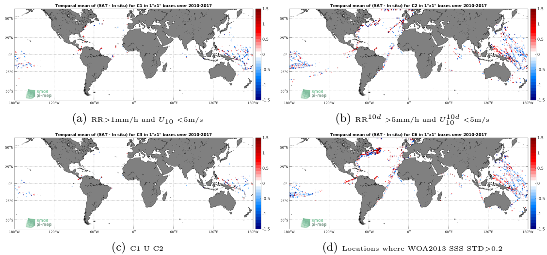
Figure 12: Temporal mean gridded over spatial boxes of size 1^\circ \times 1^\circ of \Delta SSS (SMOS-L2-DPGS-v662 - TSG-LEGOS-DM) for 4 different subdatasets corresponding to: RR > 1\text{mm/h} and U_{10} < 5\text{m/s} (a), RR^{10d} > 5\text{mm/h} and U_{10}^{10d} < 5\text{m/s} (b), C1 U C2 (c), Locations where WOA2013 SSS STD > 0.2 (d).
