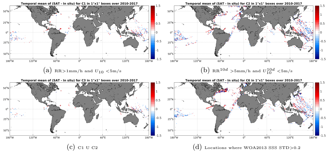
Figure 12: Temporal mean gridded over spatial boxes of size 1^\circ \times 1^\circ of \Delta SSS (SMOS-L2-DPGS-v662 - TSG-LEGOS-DM) for 4 different subdatasets corresponding to:RR >1 mm/h and U_{10} < 5 m/s (a), RR^{10d} > 5 mm/h and U_{10}^{10d} < 5 m/s (b), C1 U C2 (c),Locations where WOA2013 SSS STD >0.2 (d).
