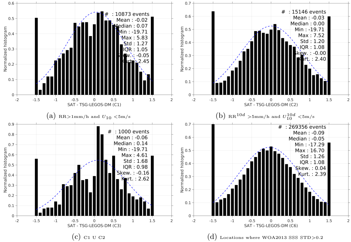
Figure 13: Normalized histogram of \Delta\text{SSS} (SMOS-L2-DPGS-v662 - TSG-LEGOS-DM) for 6 different subdatasets corresponding to: RR > 1mm/h and U_{10} < 5\text{m/s} (a), RR^{10d} > 5\text{mm/h} and U_{10}^{10d} < 5\text{m/s} (b), C1 U C2 (c), Locations where WOA2013 SSS STD > 0.2 (d).
