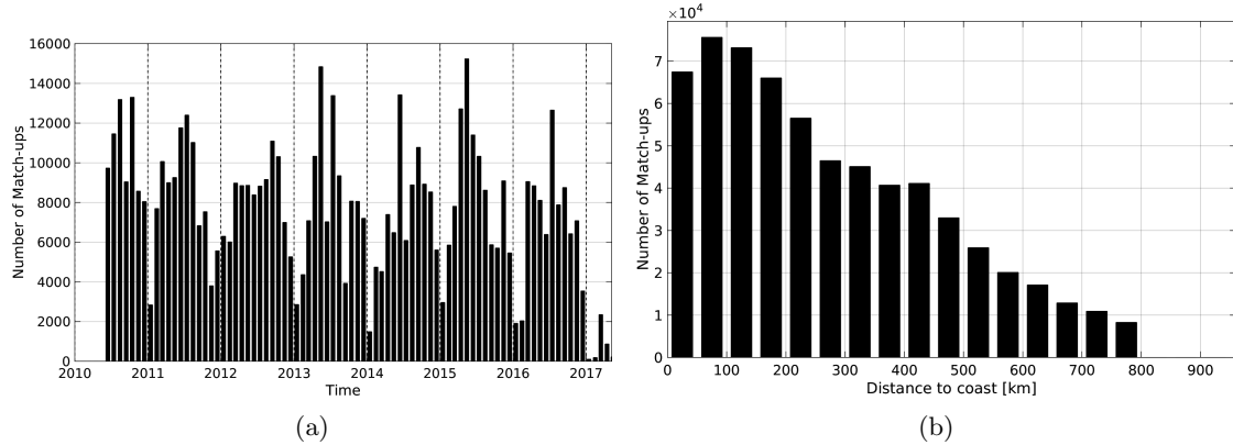
Figure 1: Number of match-ups between TSG-LEGOS-DM and SMOS-L2-DPGS-v662 SSS as a function of time (a) and as function of the distance to coast (b) over the SMOS coastal zone ( \approx 800 km) 60N-60S Pi-MEP region and for the full satellite product period.
