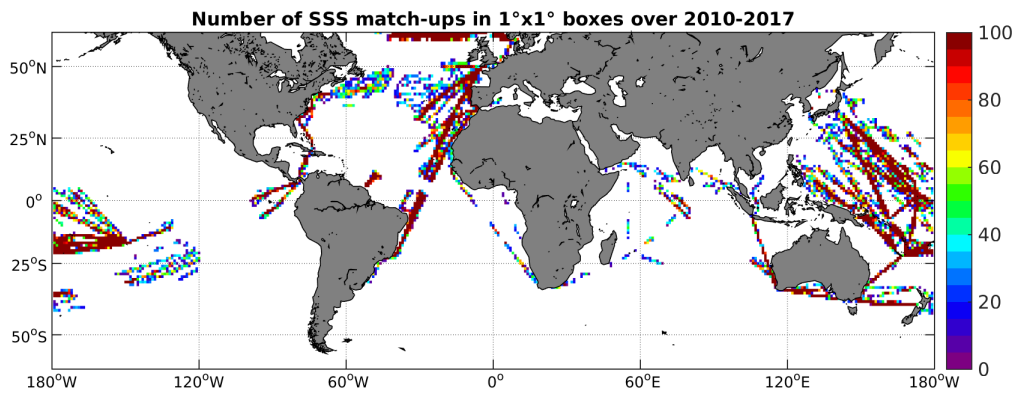
Figure 4: Number of SSS match-ups between TSG-LEGOS-DM SSS and the SMOS-L2-DPGS-v662 SSS product for the SMOS coastal zone ( \pm 800\text{km} ) 60N-60S Pi-MEP region over 1^\circ \times 1^\circ boxes and for the full satellite product period.
