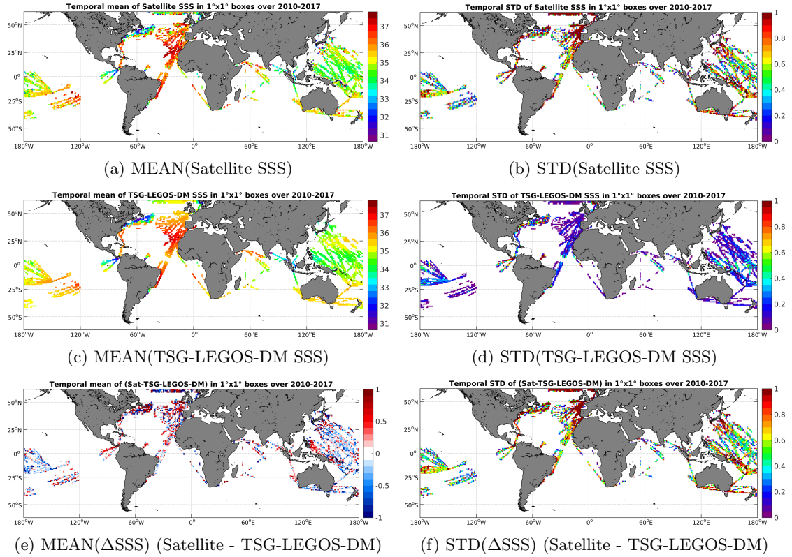
Figure 6: Temporal mean (left) and STD (right) of SSS from SMOS-L2-DPGS-v662 (top), TSG-LEGOS-DM (middle), and of \Delta SSS (Satellite - TSG-LEGOS-DM). Only match-up pairs are used to generate these maps.
