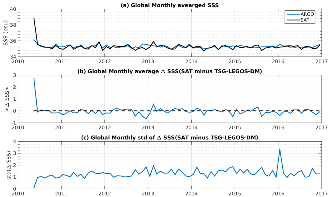
Figure 7: Time series of the monthly averaged mean SSS (top), mean \Delta SSS (Satellite - TSG-LEGOS-DM) and STD of \Delta SSS (Satellite - TSG-LEGOS-DM) over the SMOS coastal zone ( \approx 800 km) 60N-60S Pi-MEP region considering all match-ups collected by the Pi-MEP platform.
