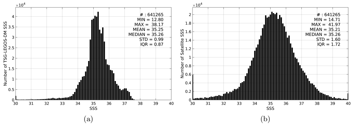
Figure 2: Histograms of SSS from TSG-LEGOS-DM (a) and SMOS-L2-DPGS-v662 (b) considering all match-up pairs per bins of 0.1 over the SMOS coastal zone ( \approx 800 km) 60N-60S Pi-MEP region and for the full satellite product period.
