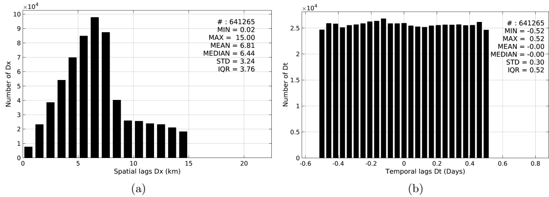
Figure 5: Histograms of the spatial (a) and temporal (b) lags between the time of the TSG-LEGOS-DM measurements and the date of the corresponding SMOS-L2-DPGS-v662 SSS product.
