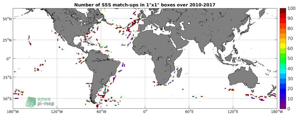
Figure 4: Number of SSS match-ups between TSG (GOSUD-Sailing-ship) SSS and the SMOS SSS L2 v662 (ESA) SSS product for the SMOS coastal zone (<800km) 60N-60S Pi-MEP region over 1^\circ \times 1^\circ boxes and for the full satellite product period.
