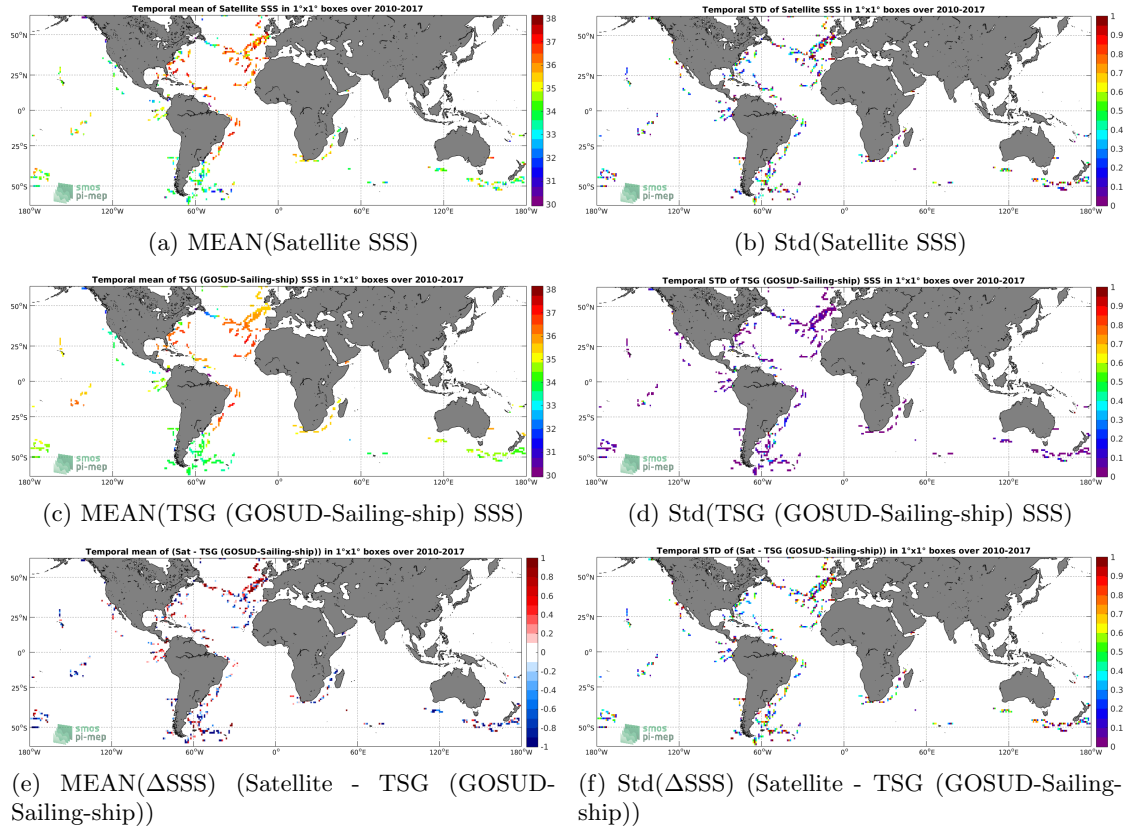
Figure 6: Temporal mean (left) and Std (right) of SSS from SMOS SSS L2 v662 (ESA) (top), TSG (GOSUD-Sailing-ship) (middle), and of \Delta SSS (Satellite - TSG (GOSUD-Sailing-ship)). Only match-up pairs are used to generate these maps.
