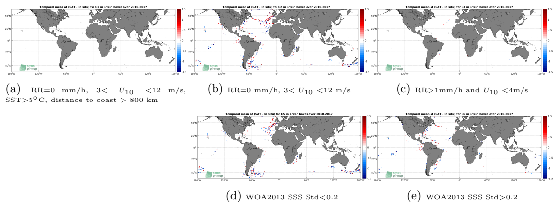
Figure 12: Temporal mean gridded over spatial boxes of size 1^\circ \times 1^\circ of \Delta\text{SSS} (SMOS SSS L2 v662 (ESA) - TSG (GOSUD-Sailing-ship)) for 5 different subdatasets corresponding to:RR=0 mm/h, 3 < U_{10} < 12 m/s, SST>5°C, distance to coast > 800 km (a), RR=0 mm/h, 3 < U_{10} < 12 m/s (b), RR>1mm/h and U_{10} < 4 m/s (c), WOA2013 SSS Std<0.2 (d), WOA2013 SSS Std>0.2 (e).
