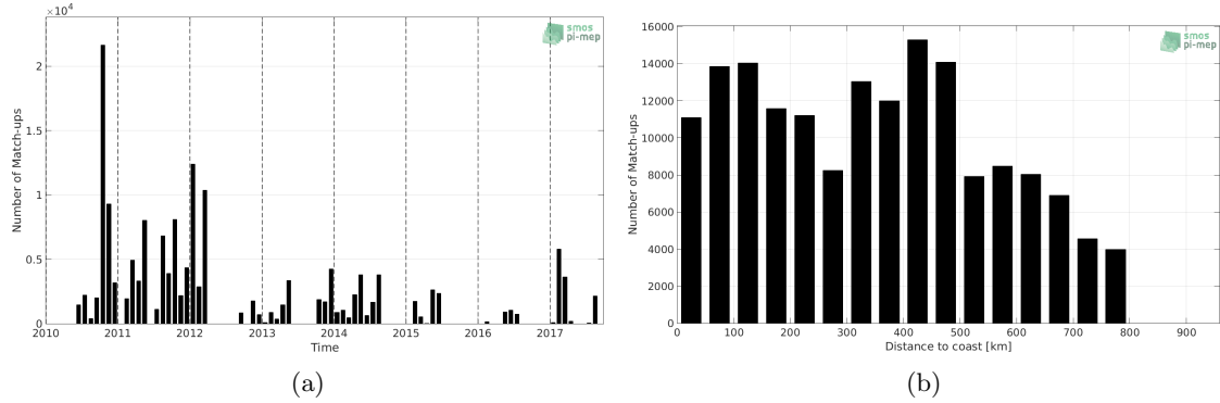
Figure 1: Number of match-ups between TSG (GOSUD-Sailing-ship) and SMOS SSS L2 v662 (ESA) SSS as a function of time (a) and as function of the distance to coast (b) over the SMOS coastal zone (<800km) 60N-60S Pi-MEP region and for the full satellite product period.
