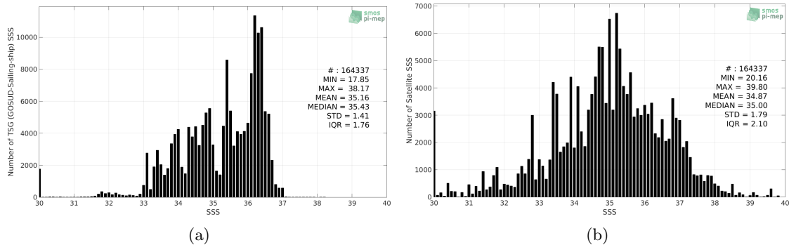
Figure 2: Histograms of SSS from TSG (GOSUD-Sailing-ship) (a) and SMOS SSS L2 v662 (ESA) (b) considering all match-up pairs per bins of 0.1 over the SMOS coastal zone (<800km) 60N-60S Pi-MEP region and for the full satellite product period.
