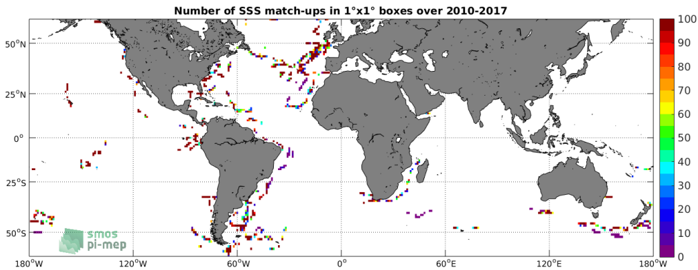
Figure 4: Number of SSS match-ups between TSG (GOSUD-Sailing-ship) SSS and the SMOS SSS L2 v662 (ESA) SSS product for the SMOS coastal zone (<800km) 60N-60S Pi-MEP region over 1°x1° boxes and for the full satellite product period.
