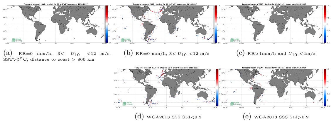
Figure 12: Temporal mean gridded over spatial boxes of size 1^\circ \times 1^\circ of \Delta SSS (SMOS SSS L2 v662 (ESA) - TSG (GOSUD-Sailing-ship)) for 5 different subdatasets corresponding to: RR=0 mm/h, 3 < U_{10} < 12 m/s, SST > 5°C, distance to coast > 800 km (a), RR=0 mm/h, 3 < U_{10} < 12 m/s (b), RR > 1mm/h and U_{10} < 4 m/s (c), WOA2013 SSS Std < 0.2 (d), WOA2013 SSS Std > 0.2 (e).
